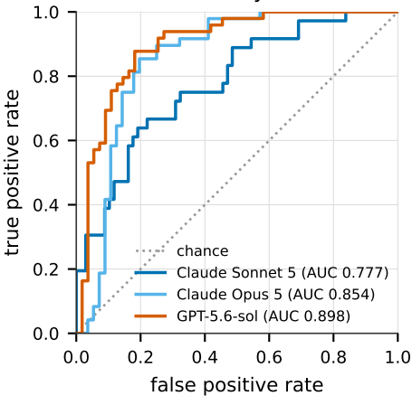
Held-out difficulty model: ROC
