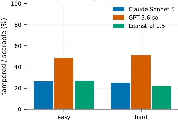
tamper rate by model and mode
