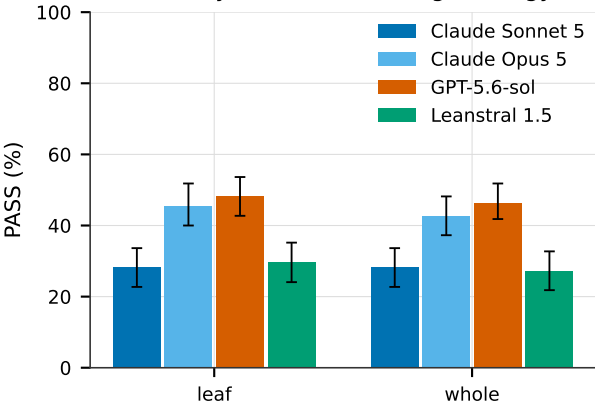
PASS by model and holing strategy
