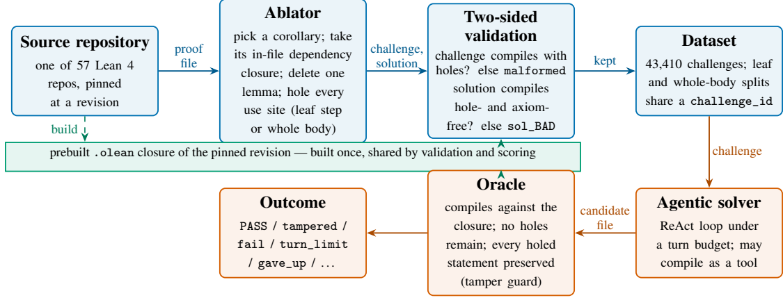
Figure 1: Dataflow of the ablation pipeline. Top row: a file from a pinned repository is ablated (one lemma deleted from a corollary’s closure, its use sites holed), and the resulting (challenge, solution) pair is kept only if both sides compile (§3.3). Bottom row: a solver rewrites the challenge and is scored by real compilation plus the hole and statement-preservation checks (§3.4, §3.5). Validation and scoring compile against the same prebuilt .olean closure, so a kept challenge is solvable and a scored answer is checked under exactly the conditions that admitted it.
