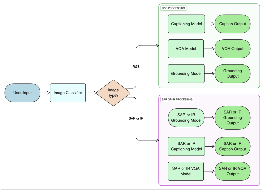
Fig. 1. System Workflow
