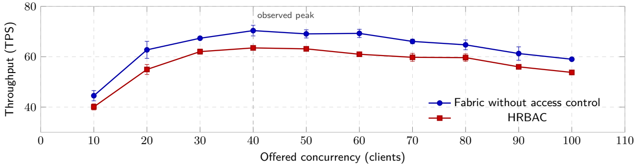
Figure 3: Mean throughput and standard deviation across five interleaved runs per concurrency level.
