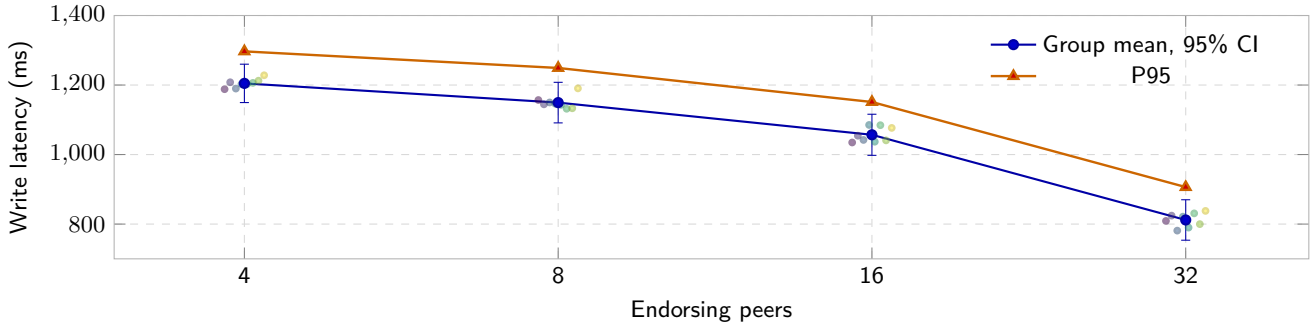
Figure 4: Run-level write latency and 95% confidence intervals by configured logical peer count.
