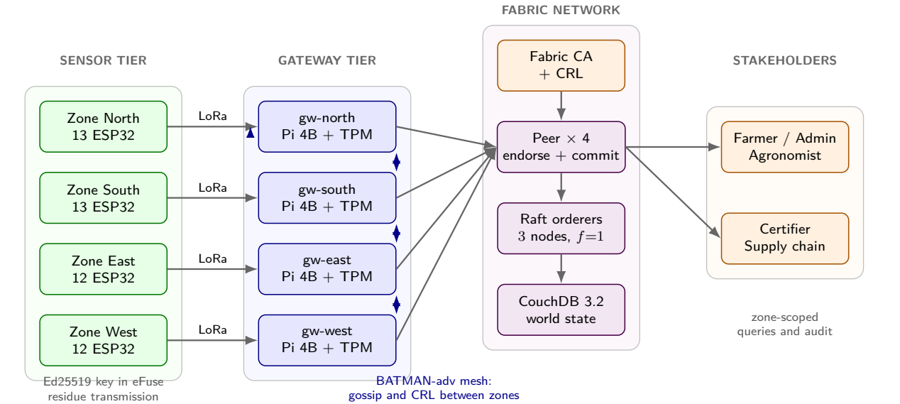
Figure 1: Deployment architecture linking sensors, zone gateways, Fabric services, and authorized users.
