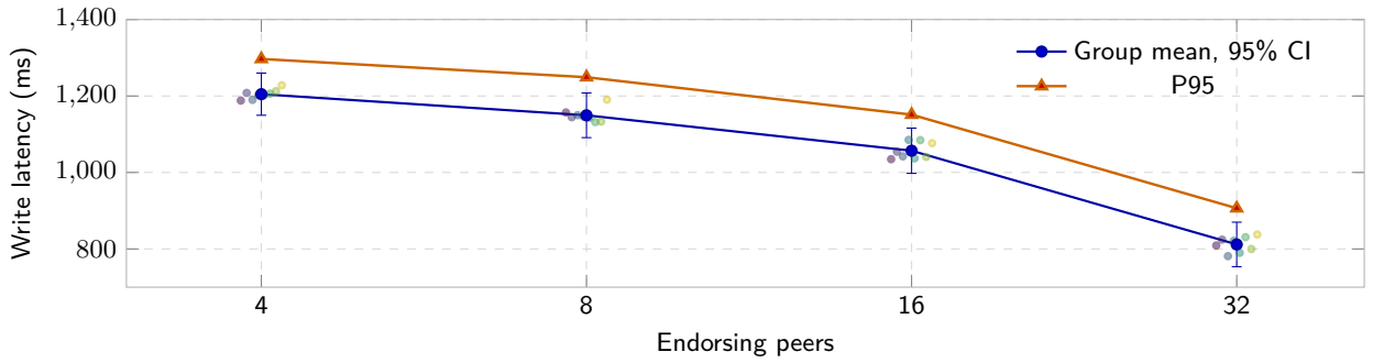
Figure 4: Run-level write latency and 95% confidence intervals by configured logical peer count.
