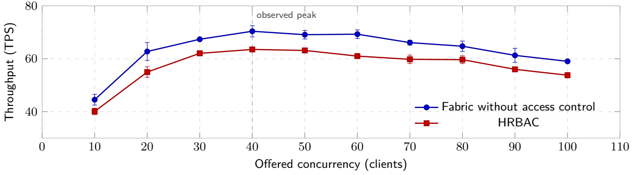
Figure 3: Mean throughput and standard deviation across five interleaved runs per concurrency level.
