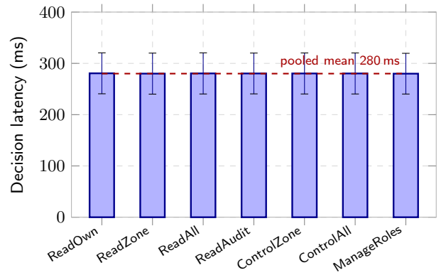
Figure 6: Policy-evaluation latency by operation type, with transaction-level standard deviations. Day-level means are equivalent within \pm 10 ms.
