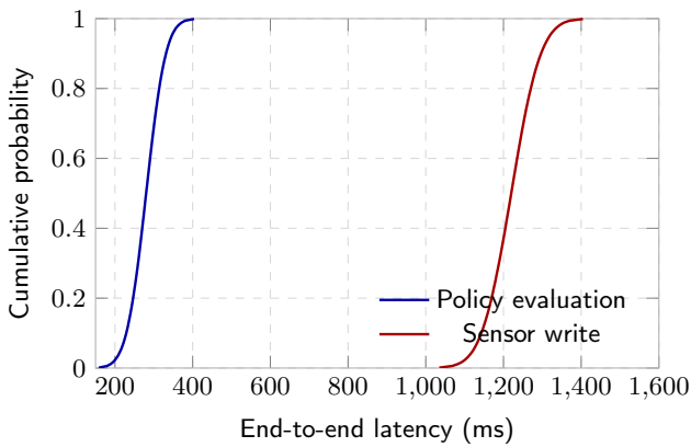
Figure 5: Empirical CDFs of the two committed transaction classes. Both traverse ordering and commitment; the horizontal gap reflects their combined differences in payload and state access.
