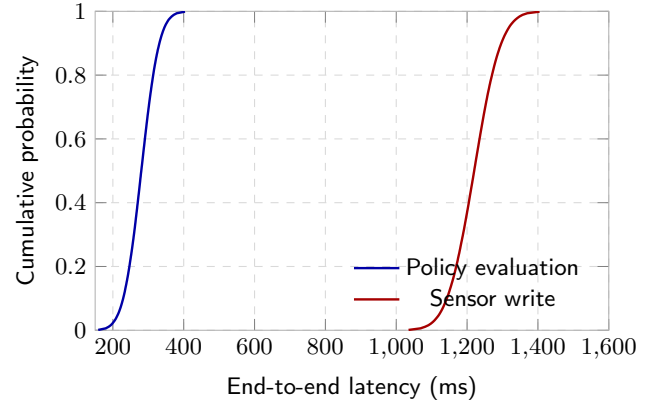
Figure 5: Empirical CDFs of the two committed transaction classes. Both traverse ordering and commitment; the horizontal gap reflects their combined differences in payload and state access.
