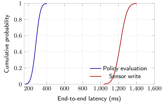
Figure 6: Empirical CDFs of the two committed transaction classes. Both traverse ordering and commitment.
