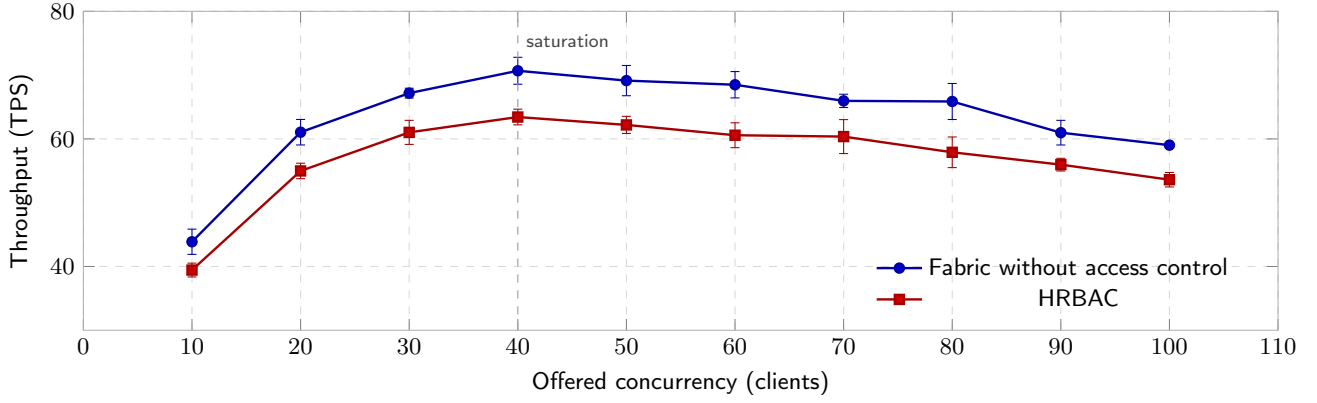
Figure 3: Throughput against offered concurrency for both arms, with standard deviations over five independent, interleaved runs per point. Both curves peak at the same offered load tested; the ten-client sampling step means the true peak could differ within that interval, and the experiment does not identify which resource saturates.
