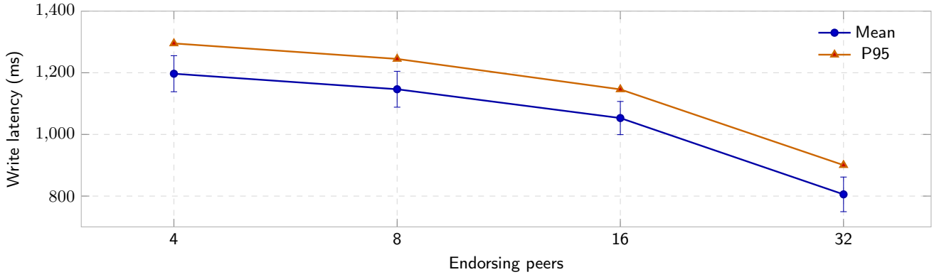
Figure 4: Write latency falls close to log-linearly with configured logical peer count ( -126.8 ms per doubling, R^2 = 0.886 ). Peer-count throughput was not measured in this design (Section 6.4); the concurrency-throughput experiment in Section 6.3 used a fixed peer configuration.
