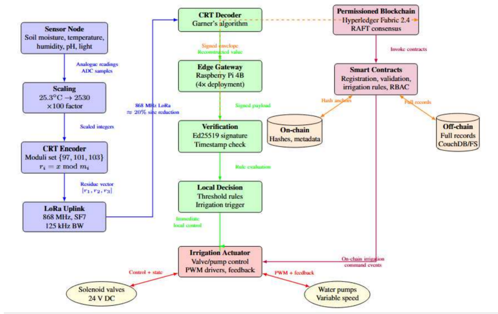
Figure 6. Gateway-side residue decoding and ledger pipeline, reproduced from [21].
