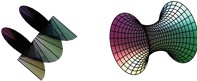
Fig. 23.1 The helicoid (left) and the catenoid (right)
