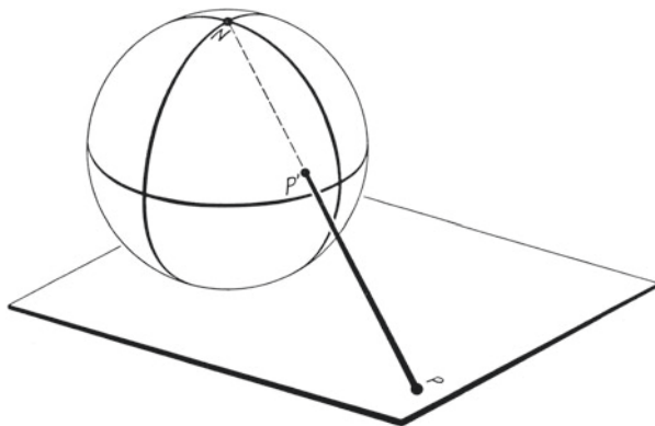
Fig. 14.1 Stereographic projection of the Riemann sphere onto the plane, Anschauliche Geometrie , 2nd edition, Springer, 1996
