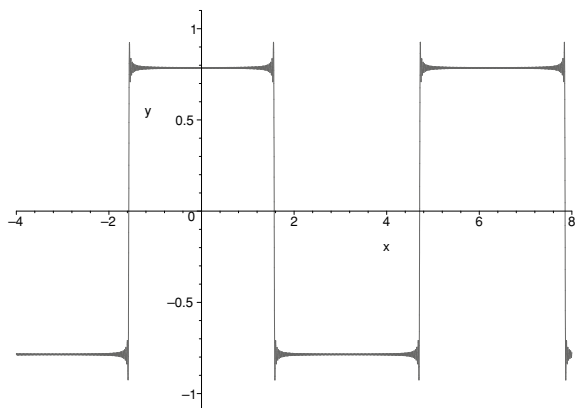
Fig. 10.2 The sum of the first 105 terms of the Fourier series for F(x) = \pm\pi/4
