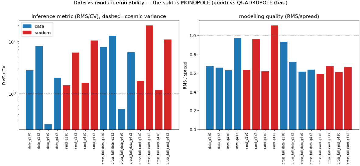
Figure 5: Per-leg within-cosmology emulability. The split is monopole (good) vs quadrupole (bad), in both data and random families. Monopoles are the inference-ready legs; the quadrupole floor is iteration-noise-limited.
