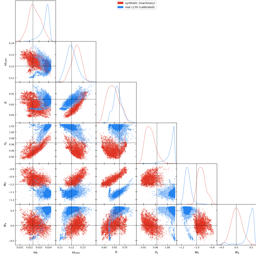
Figure 11: Broad-prior recovery of c130 over six parameters (dashed black = truth). Red: synthetic mock — recovers within 1\sigma at \chi^2/\text{dof} = 0.34 , validating the machinery over the w_0 w_a \text{CDM} + subspace. Blue: real c130 ( \chi^2/\text{dof} = 1.72 ) — \omega_{\text{cdm}}, h recovered, w_a loose (monopole-only cannot constrain the dark-energy EoS).
