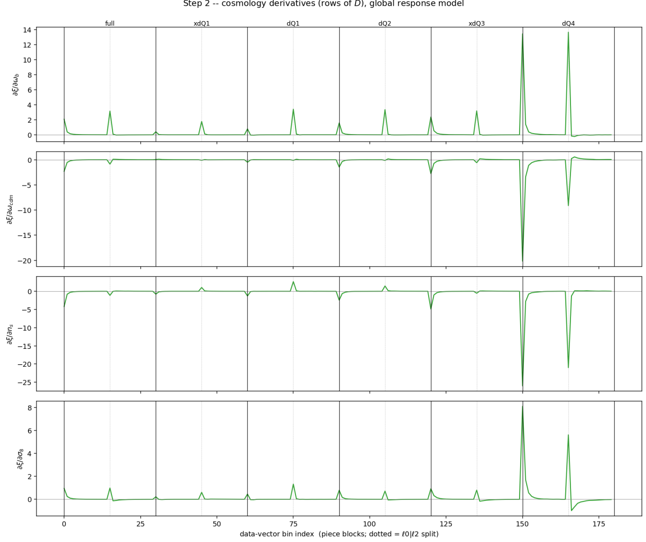
Figure 9: Step 2: the four cosmology rows of D , \partial\xi/\partial\theta , across the 180-bin vector. Solid lines separate the six pieces; dotted lines mark the \ell 0|\ell 2 split within each piece. The high-bias dQ4 piece carries the largest response.
