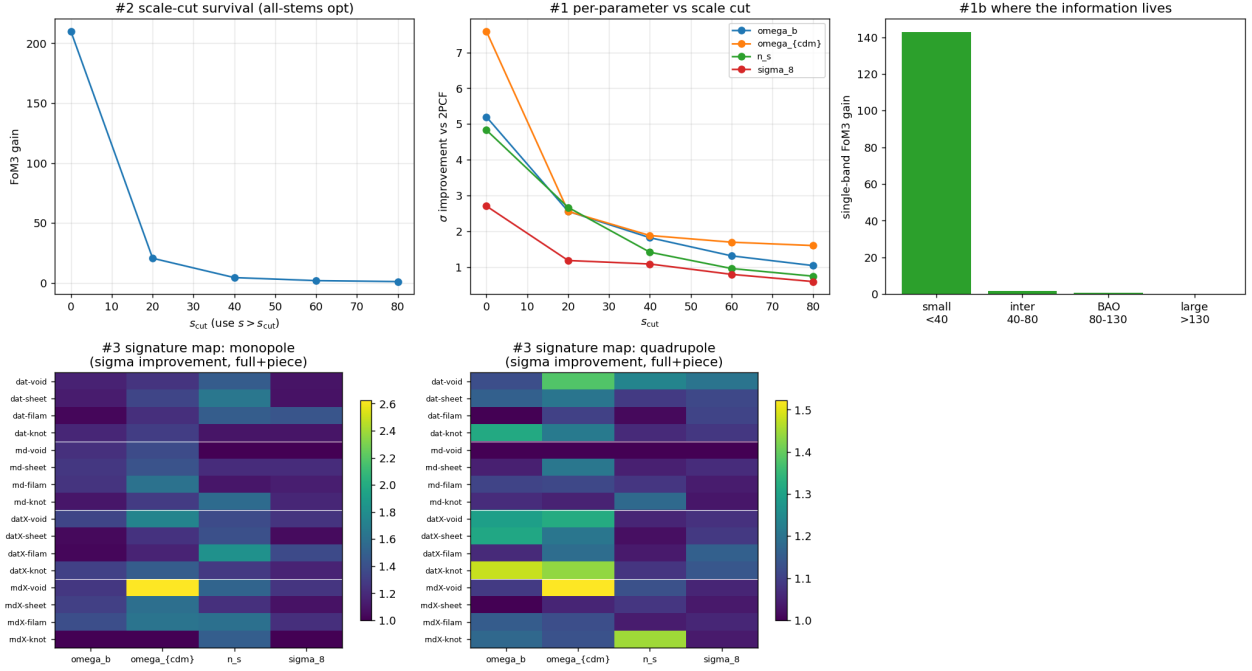
Figure 15: Top: scale-cut survival (left, FoM3; middle, per parameter) and single-band FoM3 (right) for the all-stems optimal vector — the gain is concentrated at s < 40 h^{-1} Mpc. Bottom: signature map of the per-parameter \sigma improvement from adding each (population \times environment) piece to the full auto, monopole (left) and quadrupole (right); the extreme-environment crosses dominate.
