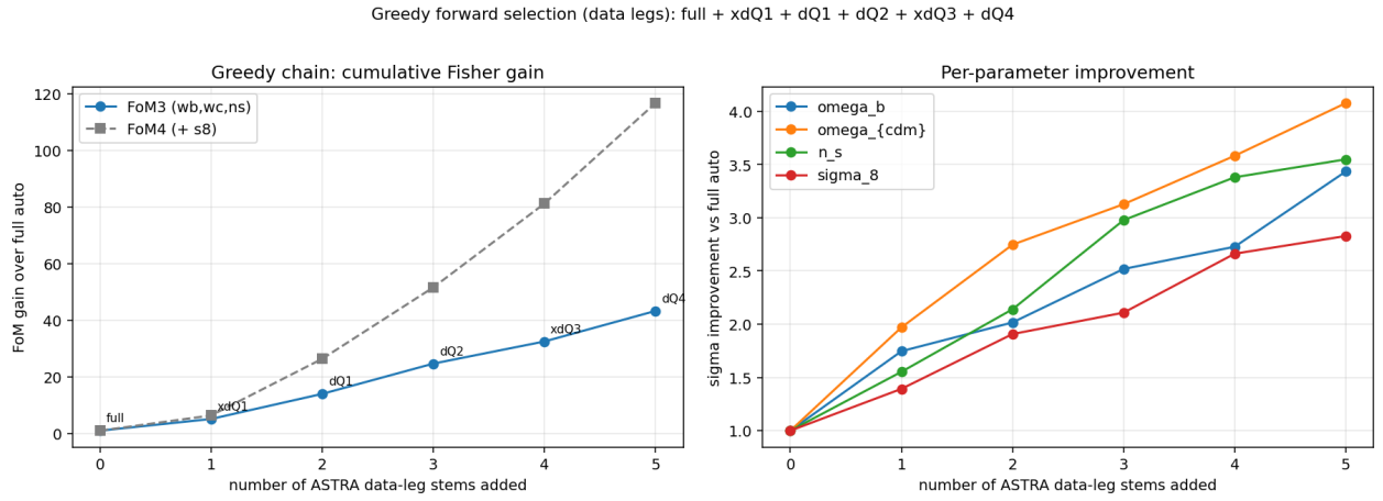
Figure 6: Greedy forward selection over the data legs. Left: cumulative FoM 3 (and FoM 4 ) gain over the full auto versus the number of ASTRA stems added — the curve flattens after \sim 4 stems. Right: per-parameter \sigma improvement over the full auto. Labels mark the stem chosen at each step.
