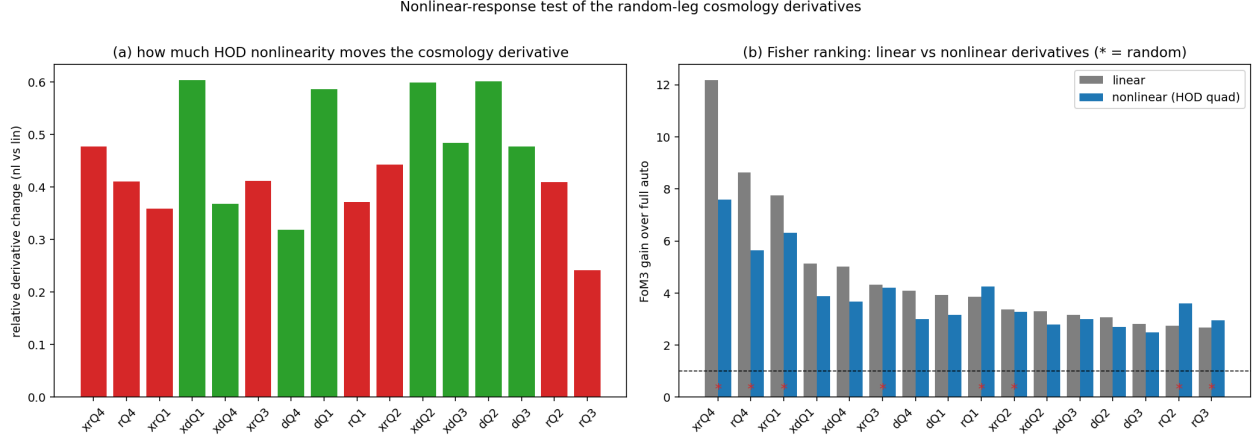
Figure 2: Test 2. (a) Relative change in the cosmology derivative when HOD nonlinearity is added to the response model: data legs (green) move as much as or more than random legs (red). (b) FoM 3 ranking with linear vs nonlinear derivatives — the random legs (*) remain on top. Nonlinearity does not single out the random legs.
