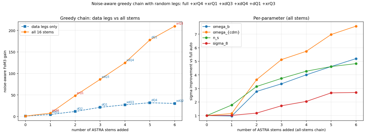
Figure 13: Left: noise-aware \text{FoM}_3 gain along the greedy chain, all sixteen stems (orange) vs data legs only (blue dashed); labels in red are random-leg picks. Right: per-parameter \sigma improvement over the full auto for the all-stems chain; \sigma_8 (red) is the flattest.
