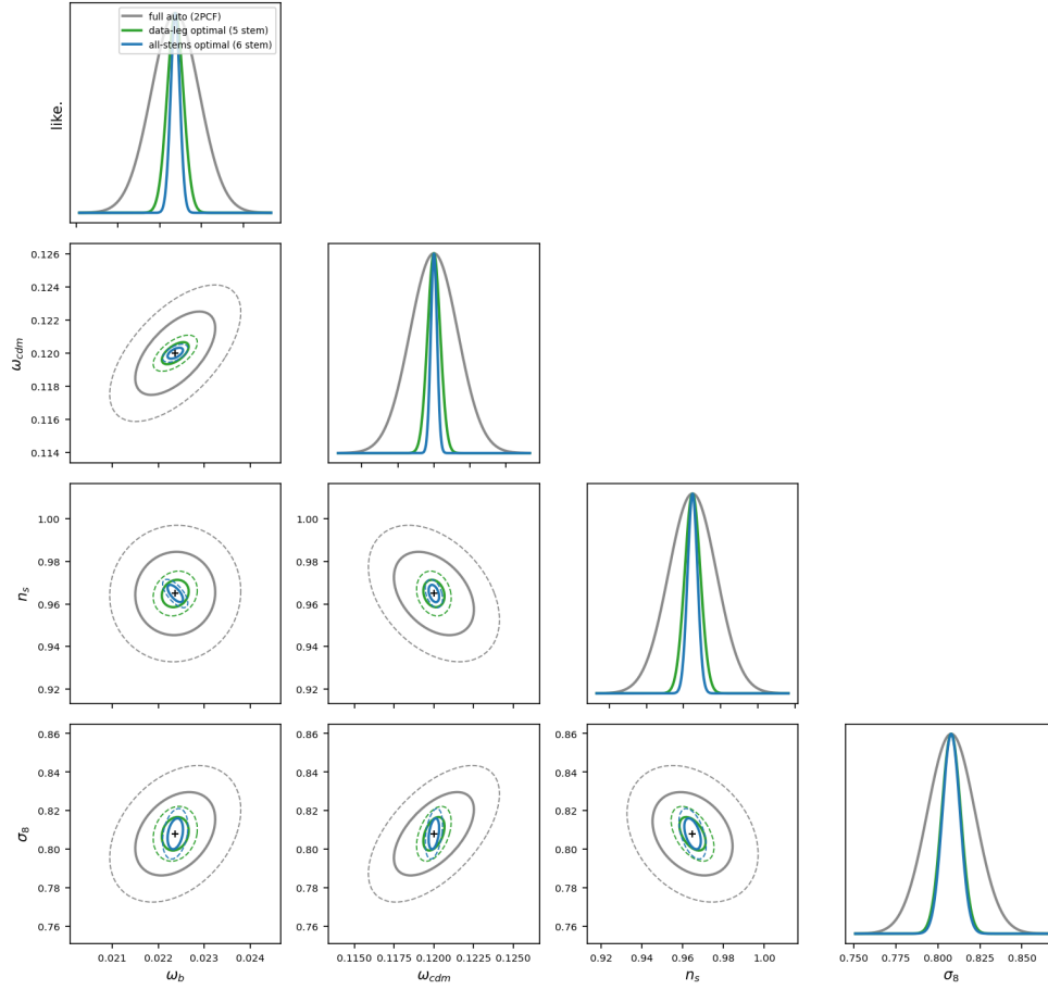
Figure 13: Updated headline forecast (noise-aware, HOD-marginalised, 68/95%): the 2PCF (grey), the data-leg optimal vector (green, FoM 3 32×), and the all-stems optimal vector (blue, FoM 3 210×). Per parameter vs the 2PCF the all-stems vector is tighter by \omega_b 5.2×, \omega_c 7.6×, n_s 4.8×, \sigma_8 2.7×. Generated by scripts/fisher_forecast_update.py .
