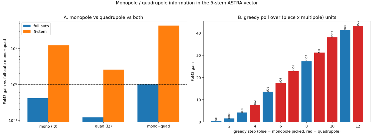
Figure 14: Left: FoM 3 gain (log scale) for mono-only, quad-only and mono+quad, for the full auto and the five-stem vector. Right: greedy poll over the twelve (piece, multipole) units; blue bars are monopole picks, red are quadrupole picks, with the cumulative FoM 3 at each step.
