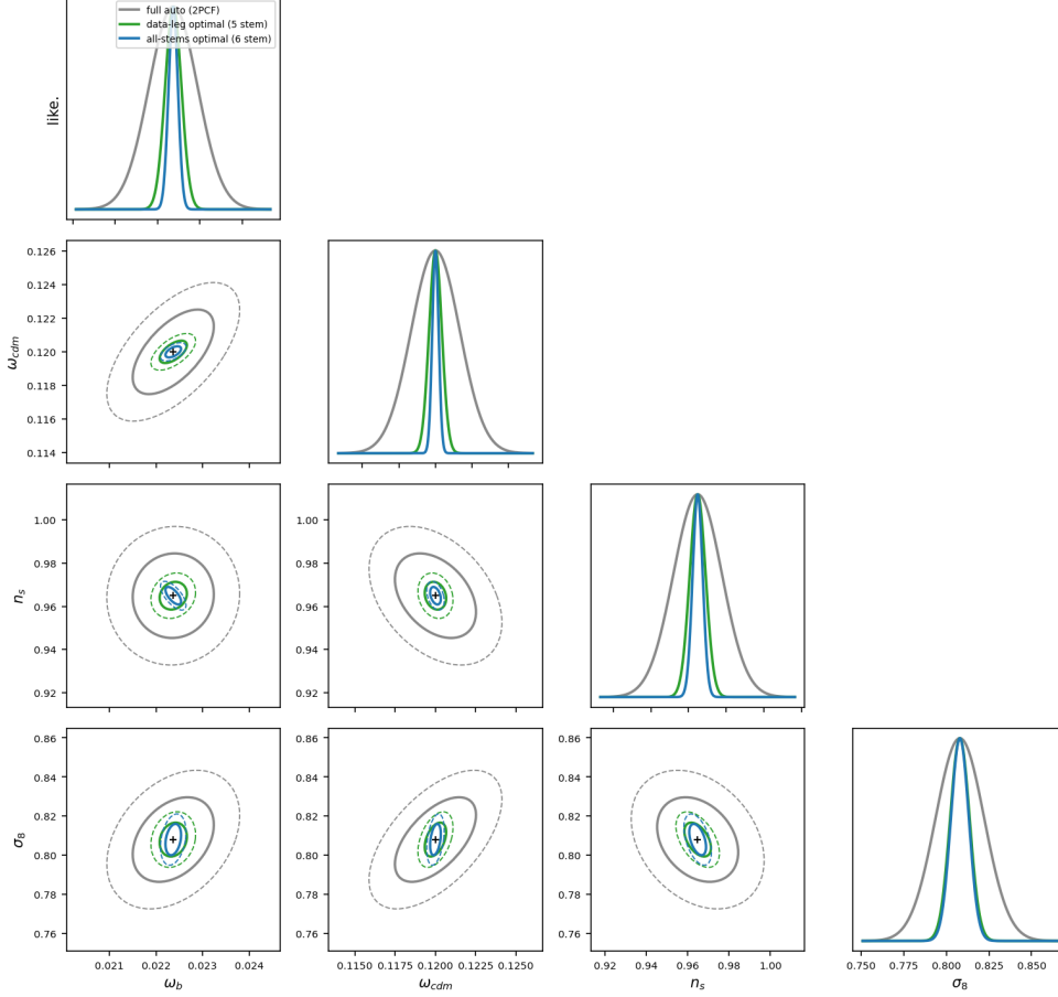
Figure 15: Updated headline forecast (noise-aware, HOD-marginalised, 68/95%): the 2PCF (grey), the data-leg optimal vector (green, FoM 3 32×), and the all-stems optimal vector (blue, FoM 3 210×). Per parameter vs the 2PCF the all-stems vector is tighter by \omega_b 5.2×, \omega_c 7.6×, n_s 4.8×, \sigma_8 2.7×. Generated by scripts/fisher_forecast_update.py .
