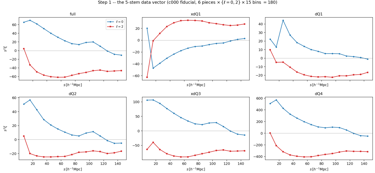
Figure 10: Step 1: the fiducial five-stem data vector, s^2 \xi_{0,2}(s) per piece. Amplitude grows void (dQ1) \rightarrow knot (dQ4).
