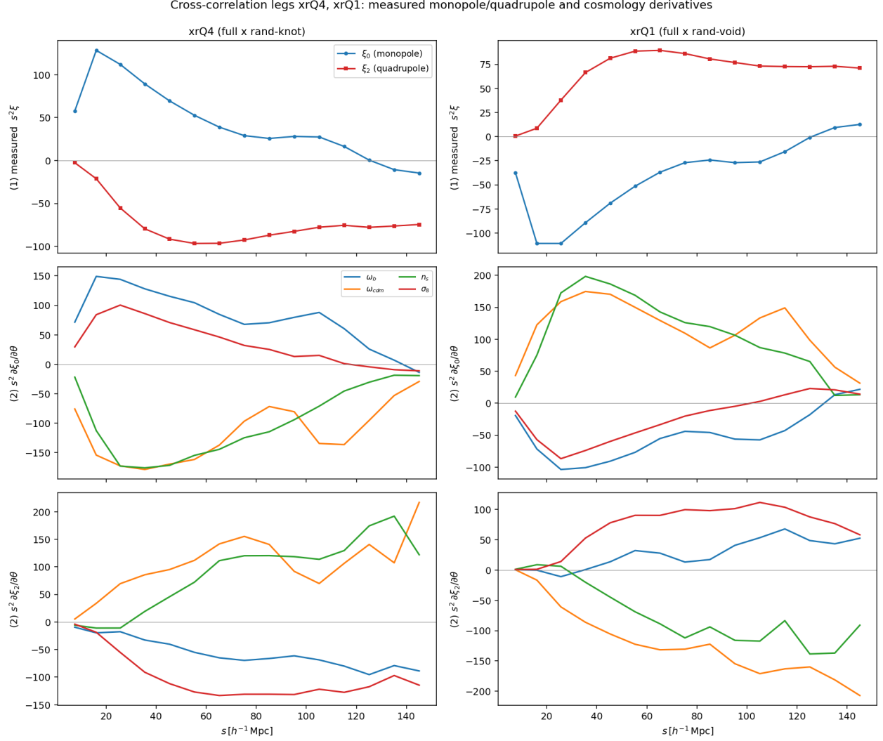
Figure 8: The two cross legs xrQ4 (knot) and xrQ1 (void). Row 1: the measured monopole and quadrupole s^2 \xi_{0,2} (c000 fiducial) — opposite in sign. Rows 2–3: the cosmology derivatives s^2 \partial \xi_{0,2} / \partial \theta — near-antisymmetric between the two legs.
