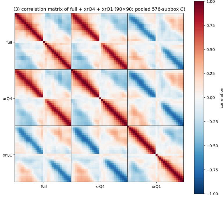
Figure 9: Correlation matrix of full+xrQ4+xrQ1 (pooled 576-subbox C ). The full – xrQ4 block is positive (red); the full – xrQ1 and xrQ4 – xrQ1 blocks are negative (blue) — the void and knot crosses are anti-correlated, hence partially independent.
