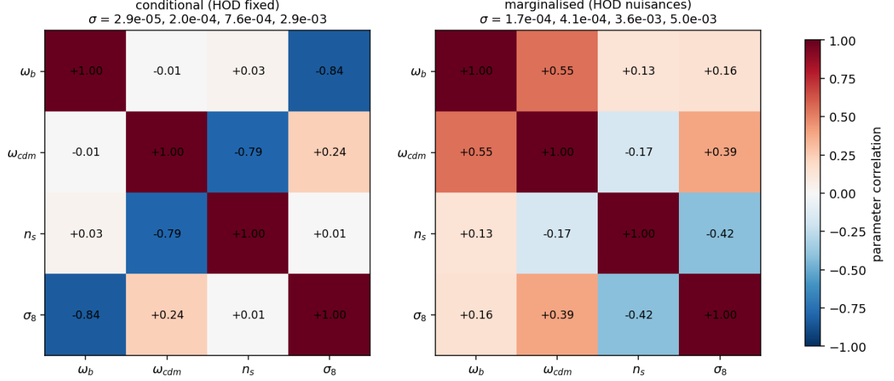
Figure 13: Step 4: cosmology parameter correlation matrices from F = D C^{-1} D^T , conditional (left) and HOD-marginalised (right), with the per-parameter \sigma in the titles. HOD marginalisation both inflates the errors and re-shapes the degeneracies.
