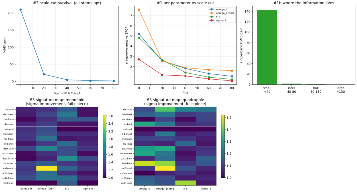
Figure 17: Top: scale-cut survival (left, FoM3; middle, per parameter) and single-band FoM3 (right) for the all-stems optimal vector — the gain is concentrated at s < 40 h^{-1} Mpc. Bottom: signature map of the per-parameter \sigma improvement from adding each (population \times environment) piece to the full auto, monopole (left) and quadrupole (right); the extreme-environment crosses dominate.
