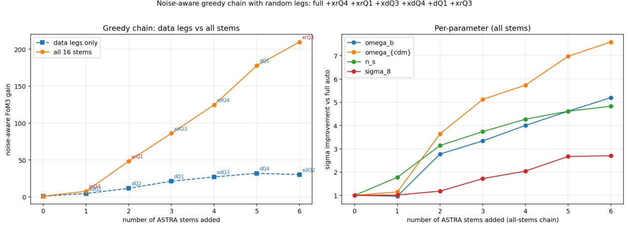
Figure 16: Left: noise-aware FoM 3 gain along the greedy chain, all sixteen stems (orange) vs data legs only (blue dashed); labels in red are random-leg picks. Right: per-parameter \sigma improvement over the full auto for the all-stems chain; \sigma_8 (red) is the flattest.
