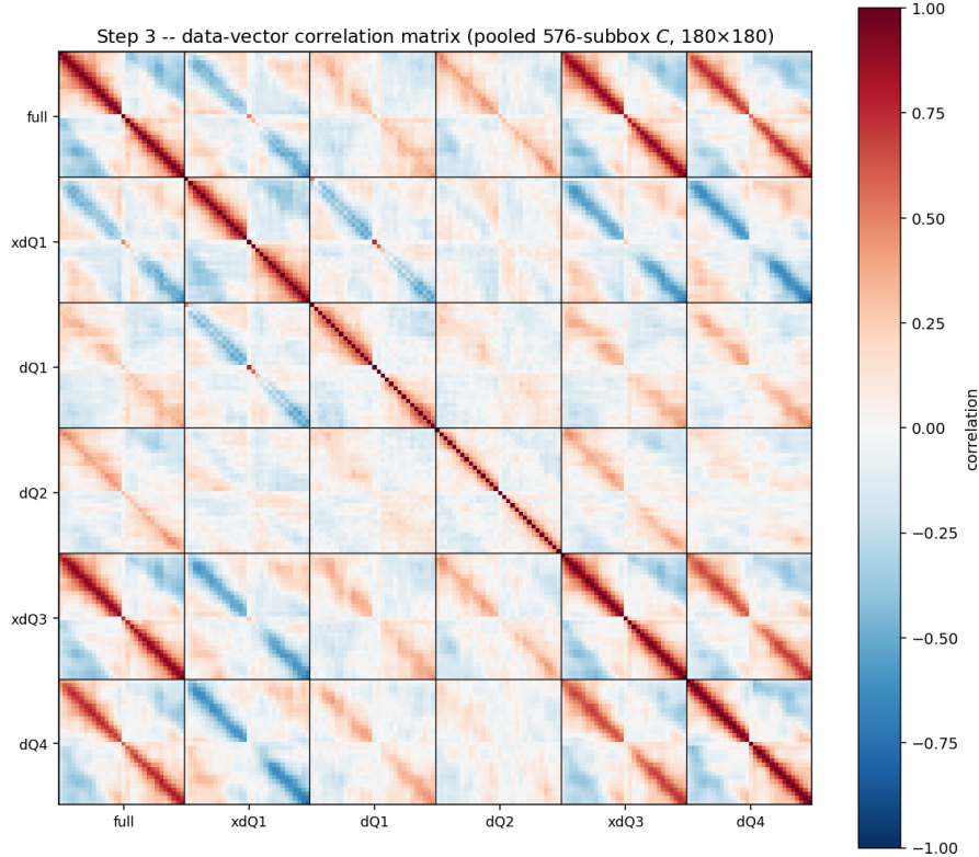
Figure 12: Step 3: the 180 \times 180 data-vector correlation matrix (pooled 576-subbox C ). Black lines separate the six pieces. Strong cross-piece correlations (e.g. full with the \mathbf{xd} crosses) are the redundancy that limits the cumulative gain.
