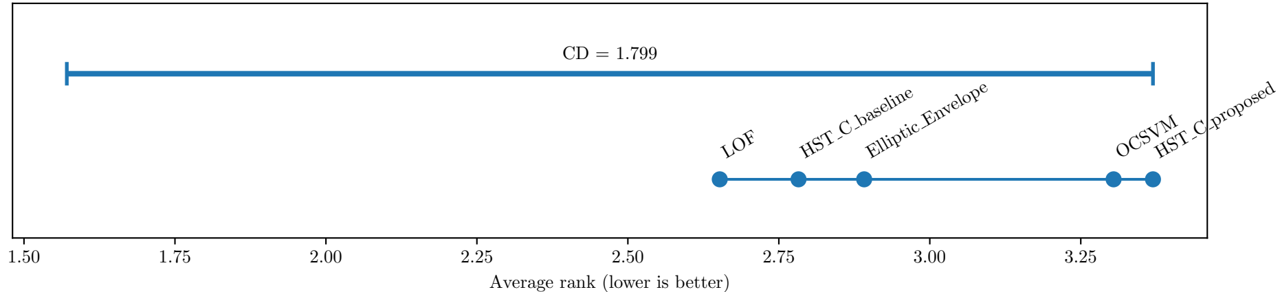
Nemenyi CD diagram (ROC AUC), N=23, k=5, Friedman p=0.415
