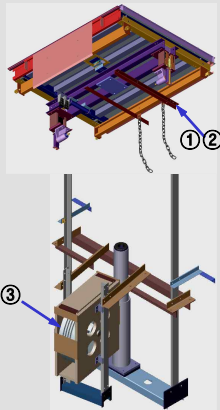
③ Compensation Sheave
