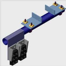
① Cable Hanger (Car)
