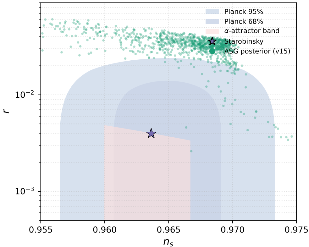
n_s - r comparison (PolyChord v15)
