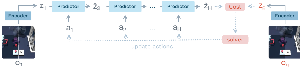
Figure 4: LeWorldModel Latent Planning. Given an initial observation \mathbf{o}_1 and a goal \mathbf{o}_g , the world model learned in Fig. 2 performs planning in the LeWM latent space. The initial state embedding \mathbf{z}_1 and the goal embedding \mathbf{z}_g are obtained from the encoder. The predictor then rolls out future latent states up to a horizon H . A latent cost between the final predicted state and the goal embedding guides a solver to optimize the action sequence. This prediction–optimization loop is repeated until convergence to a good plan candidate.
