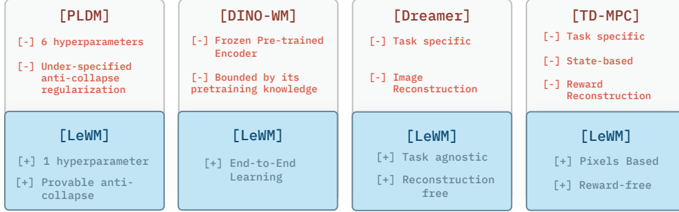
Figure 2: Characteristics of latent world model approaches. Methods are grouped by training paradigm. End-to-end methods (PLDM) learn both the encoder and predictor jointly from pixels without relying on pre-trained representations or heuristic tricks such as stop-gradient or exponential moving averages, but require many hyperparameters and lack formal collapse guarantees. Foundation-based methods (DINO-WM) avoid collapse by freezing a pre-trained foundation vision encoder, forgoing end-to-end learning. Task-specific methods (Dreamer, TD-MPC) require reward signals or privileged state access during training. LeWM addresses the limitations of each category: it is end-to-end, task-agnostic, pixel-based, reconstruction- and reward-free, and requires only a single hyperparameter with provable anti-collapse guarantees.
