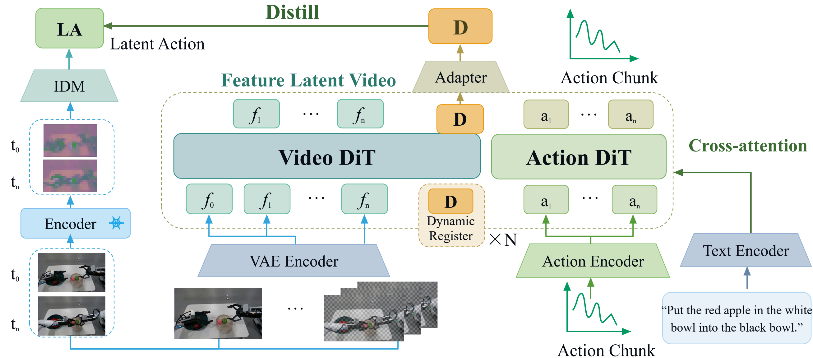
(a) ForeWAM architecture
