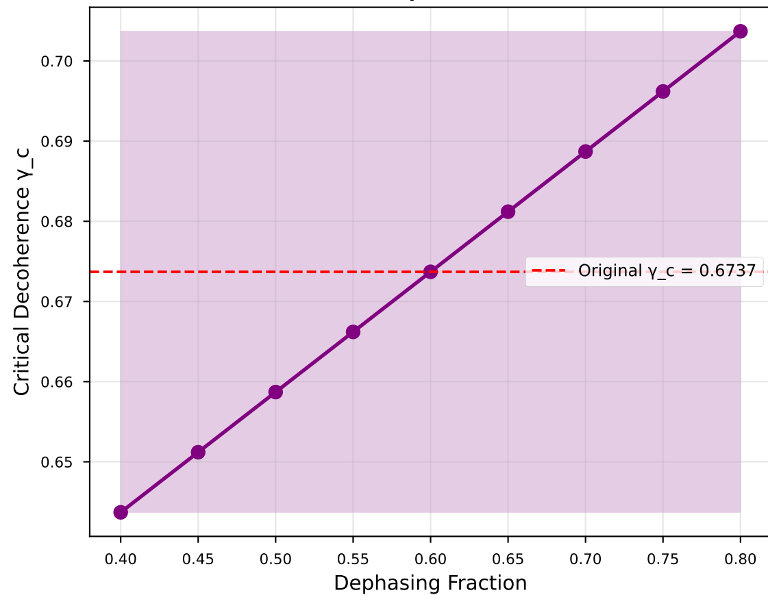
(a) Sensitivity to Noise Model
