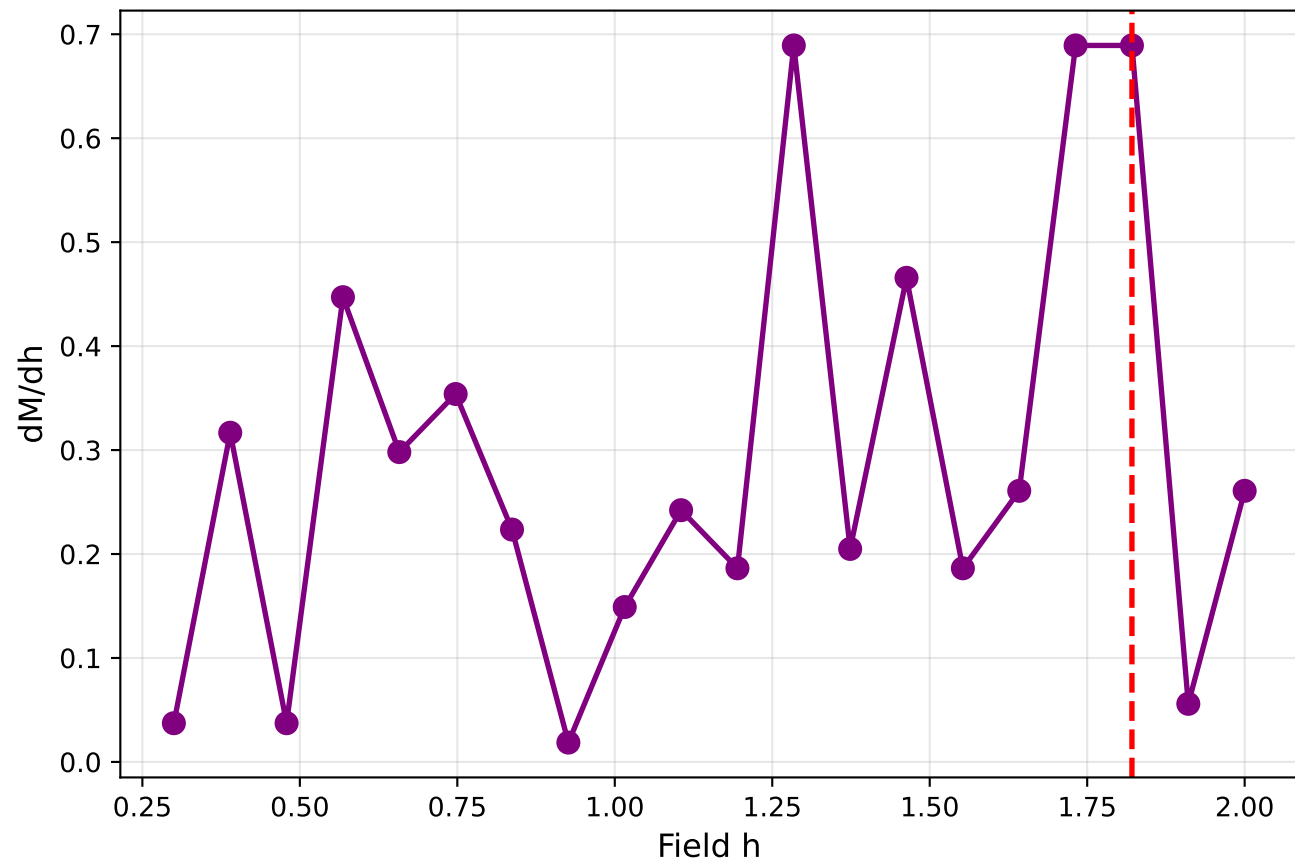
\kappa = 2.41
