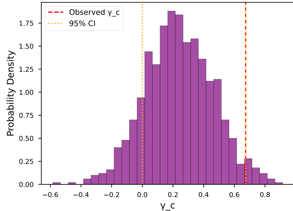
(c) Bootstrap Distribution
