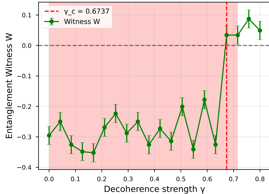
(a) Witness with 95% CI
