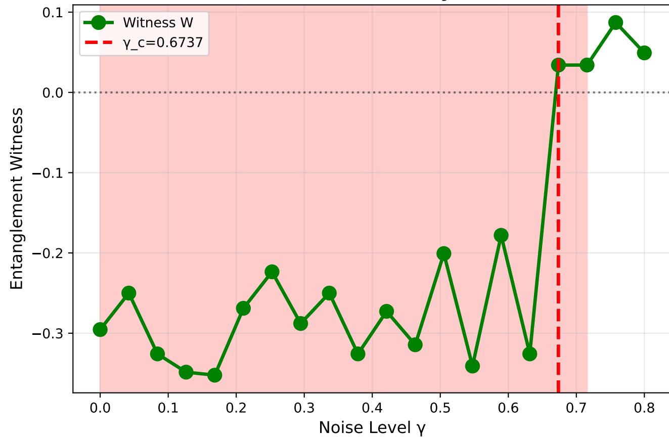
E3: Information→Physics ⚡
