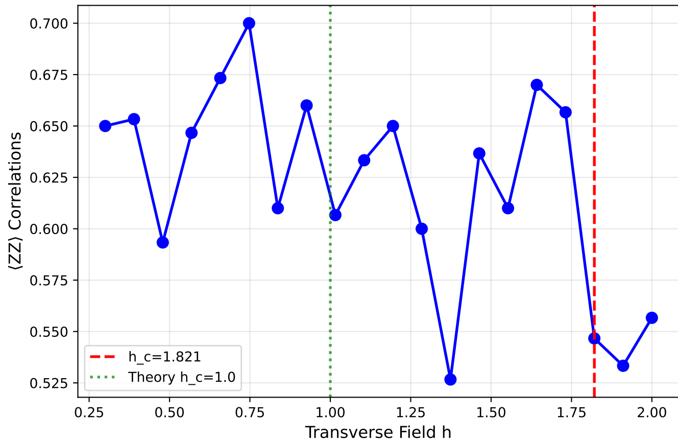
E5: Quantum Phase Transition
