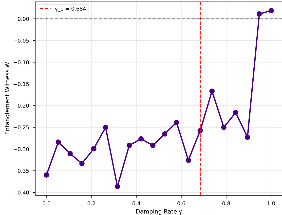
(a) GHZ State Decoherence
