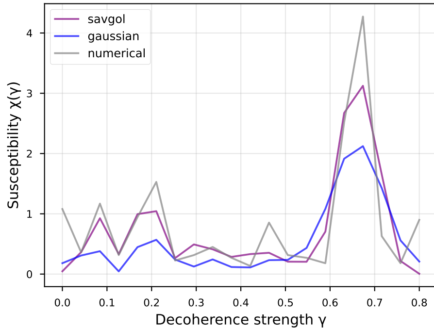
(b) Robustness to smoothing ( \kappa = 8.58 )
