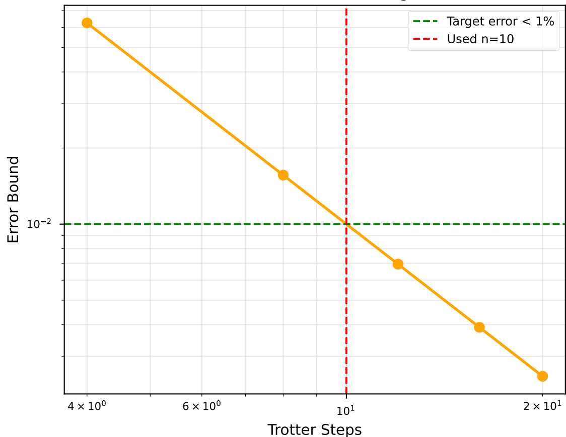
(b) Trotter Error Scaling
