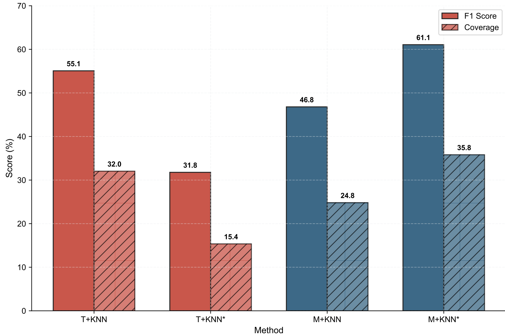
F1 Score & Coverage at PRE \geq 99% Target (50k Split, Test Set)
