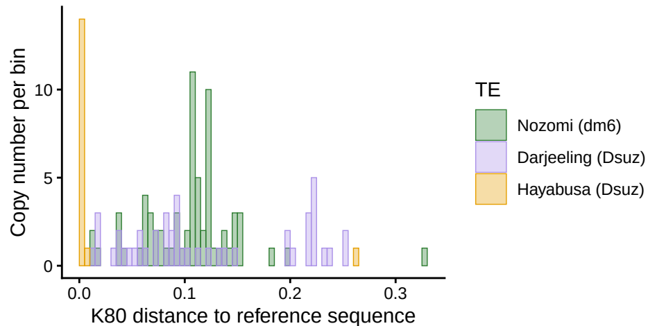
K80 values distribution for Nozomi, Darjeeling and Hayabusa insertions
