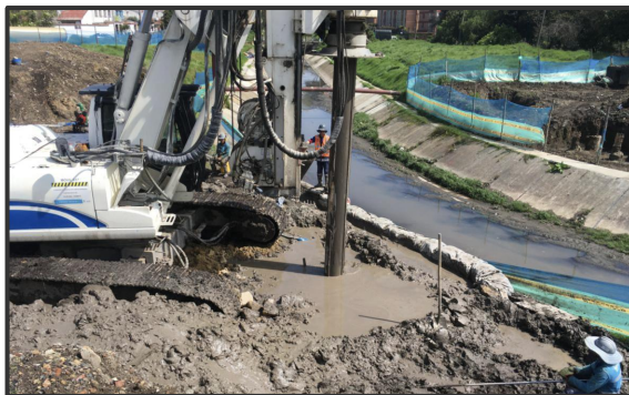
— Foundation structures: shallow and deep underground works.
