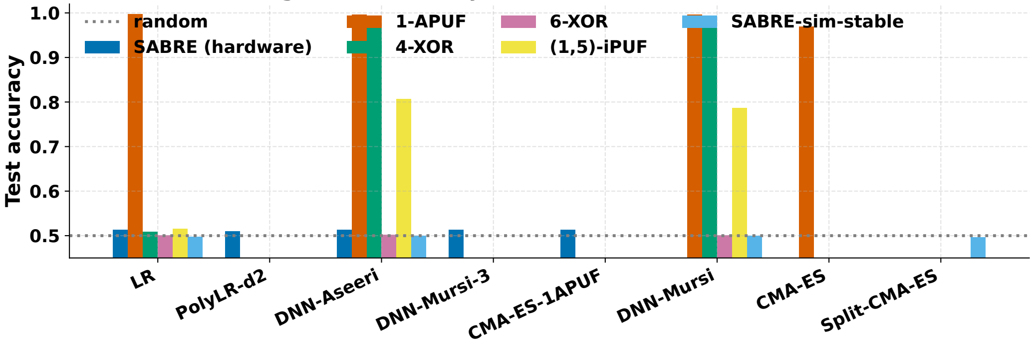
Modeling-attack accuracy: SABRE vs. hardened-APUF baselines
