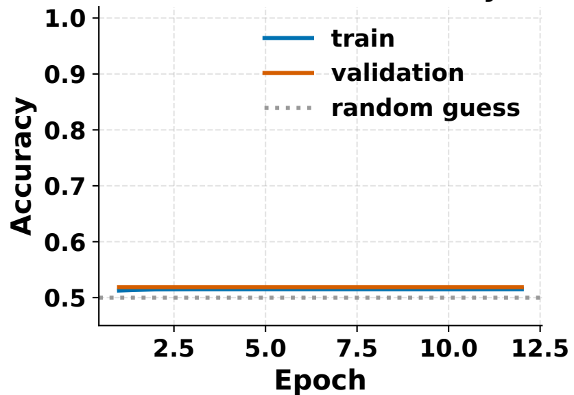
DNN-Aseeri — accuracy
