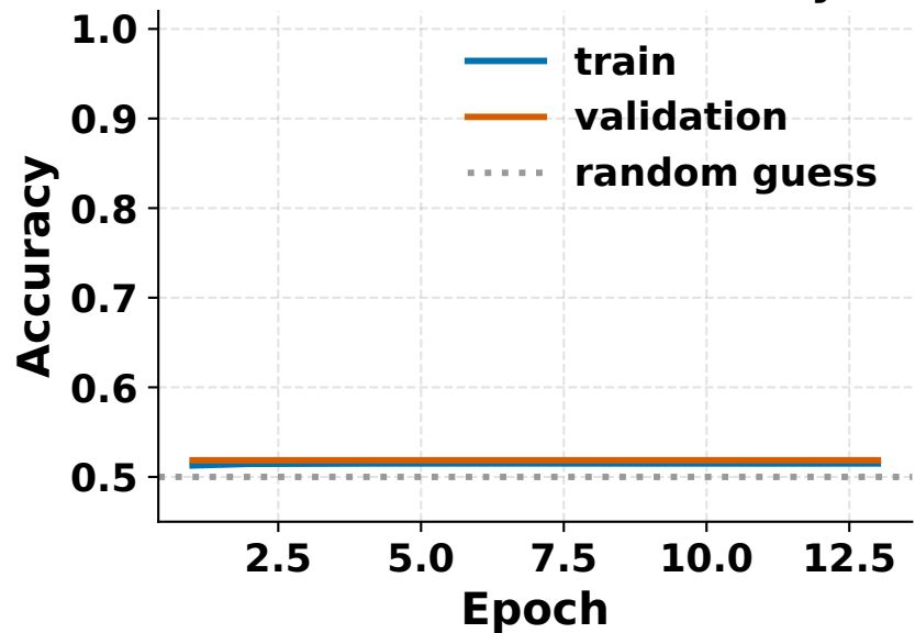
DNN-Mursi-3 — accuracy
