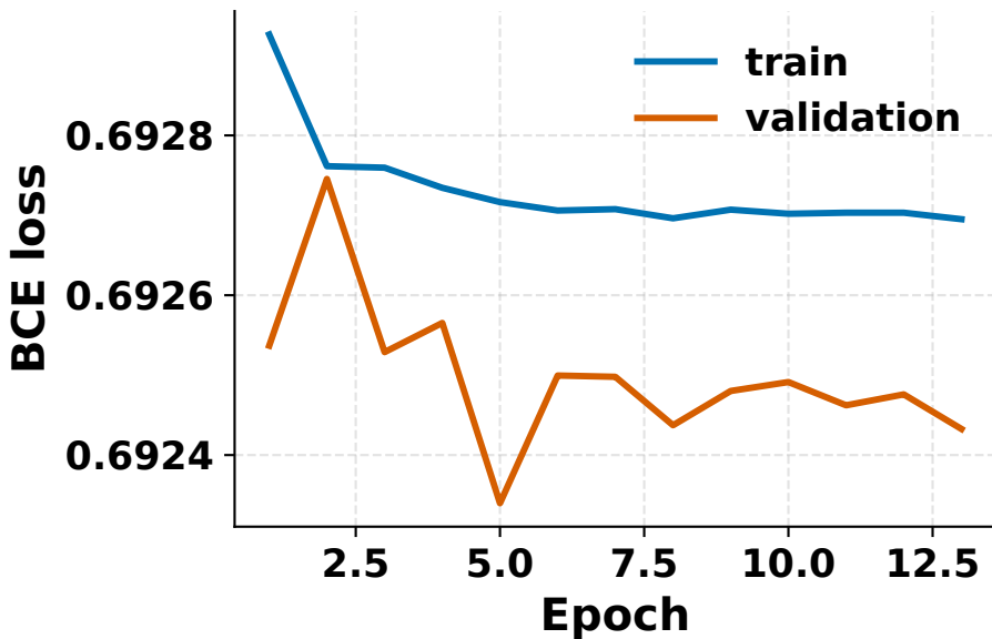
DNN-Mursi-3 — loss
