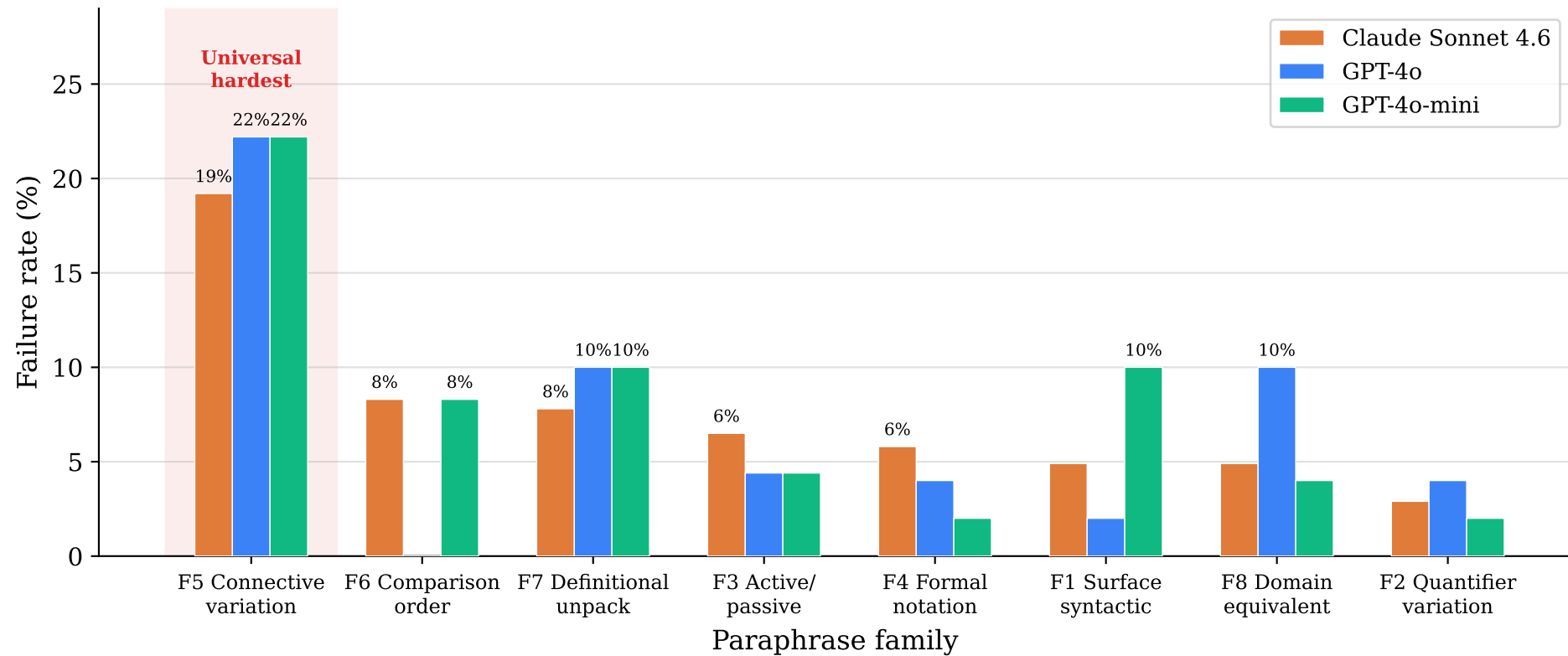
Per-family failure rates by model (Claude: 103-theorem dataset; GPT models: 50-theorem shared set)
