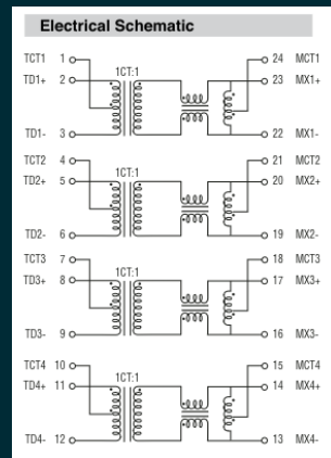
transformer datasheet
