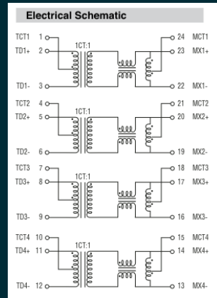
transformer datasheet
