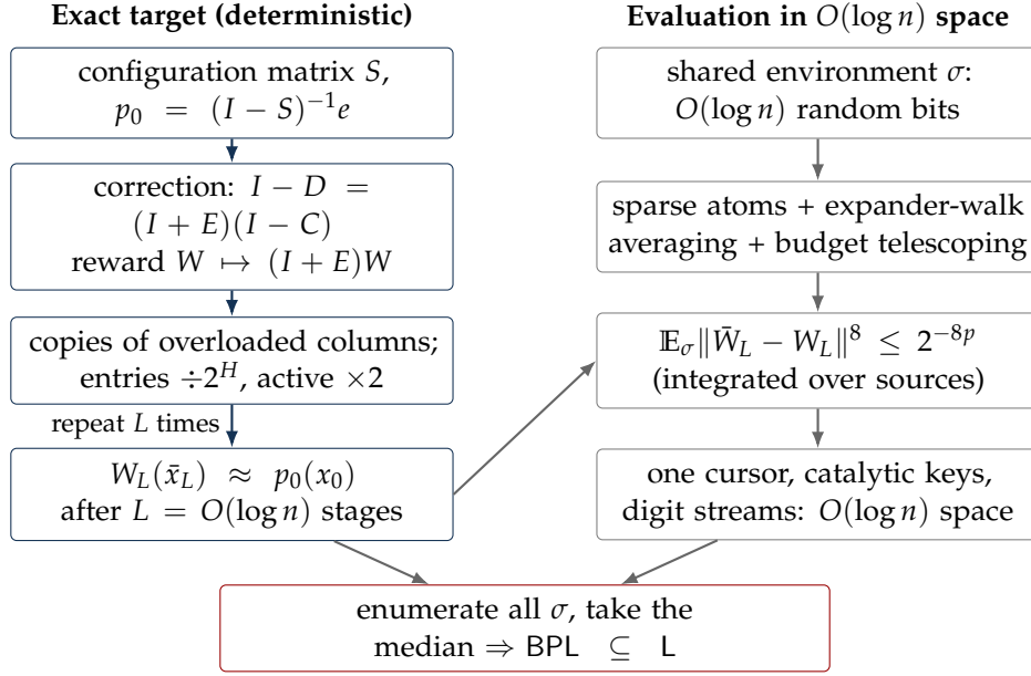
Figure 1: Architecture. The left column is Section 2; the right column is Sections 3 and 4.
