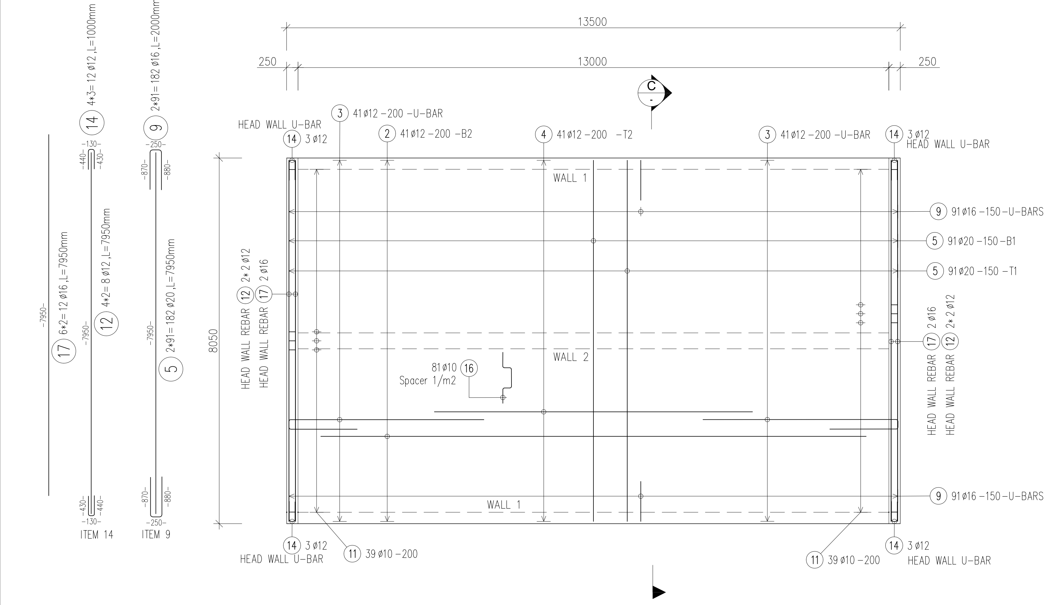
DOUBLE CELL CULVERT 01 (PLAN VIEW) TOP SLAB REINFORCEMENT DETAIL
