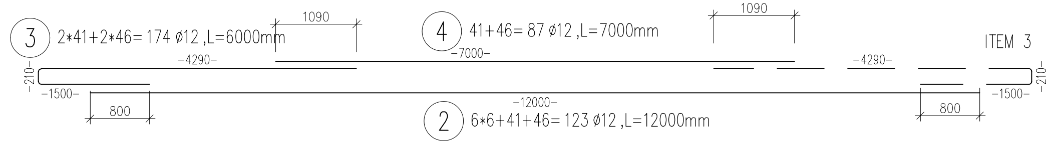
DOUBLE CELL CULVERT 01 (PLAN VIEW) BOTTOM SLAB REINFORCEMENT DETAIL
