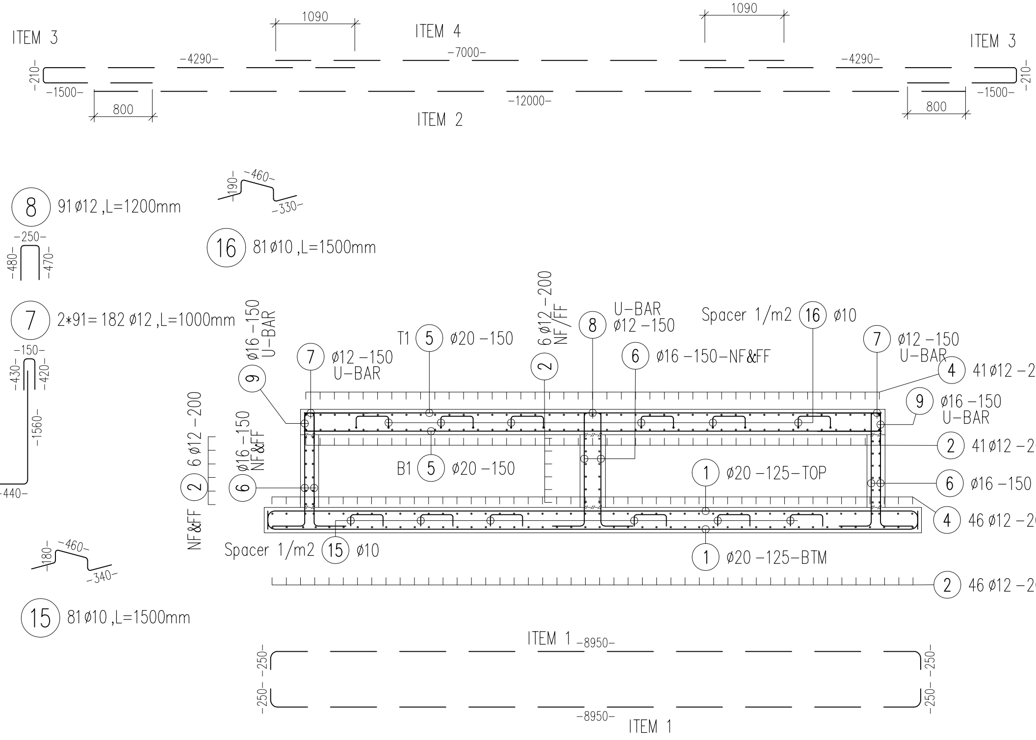
SECTION SC: 1:50
