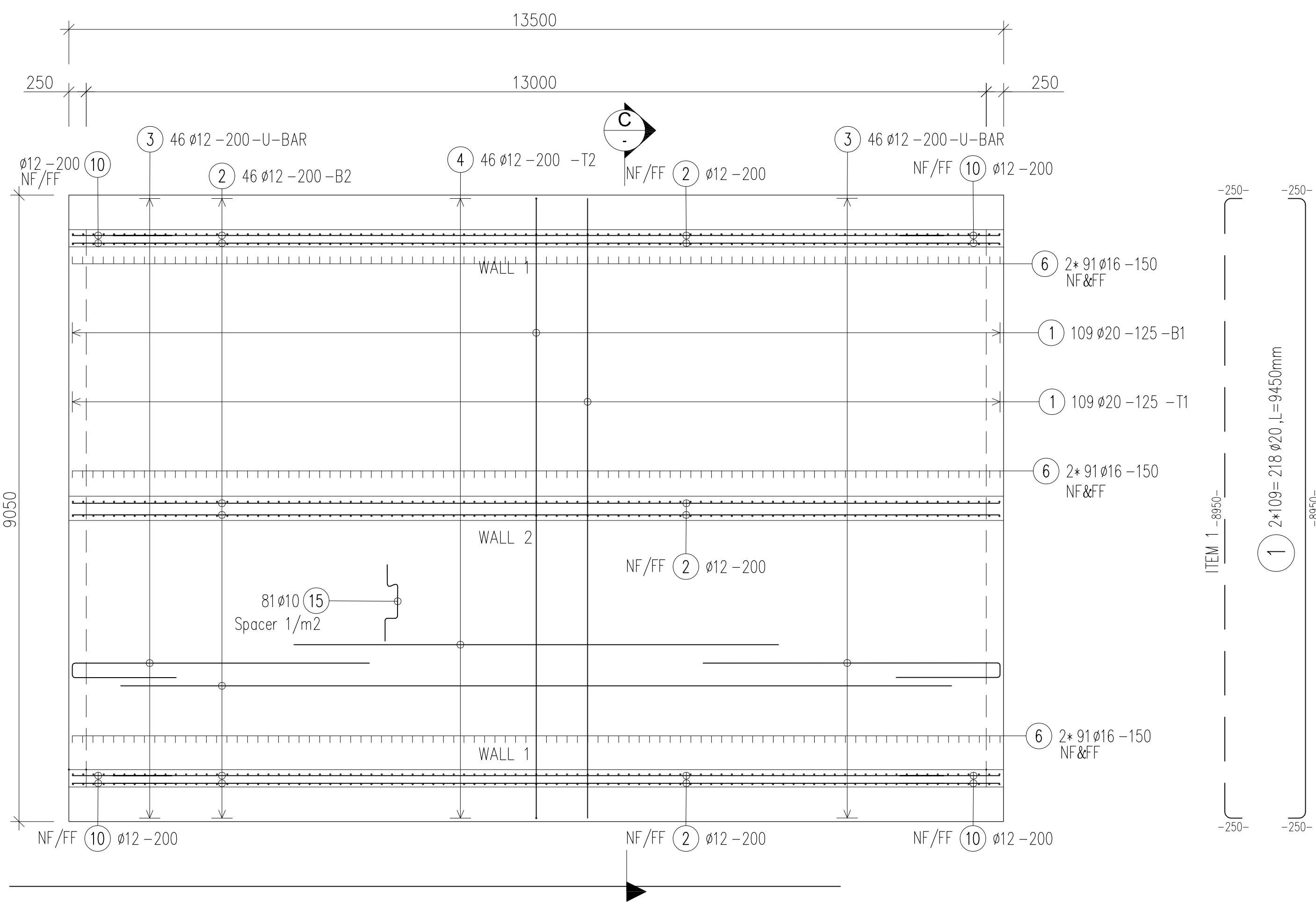
DOUBLE CELL CULVERT 01 (PLAN VIEW) BOTTOM SLAB REINFORCEMENT DETAIL
