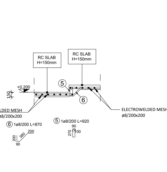
SECTION C-C 1:50
