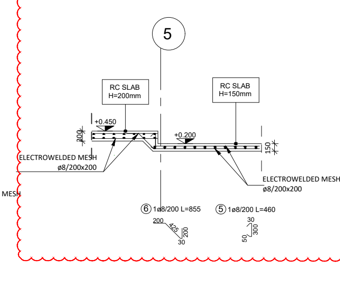
SECTION M-M 1:50
