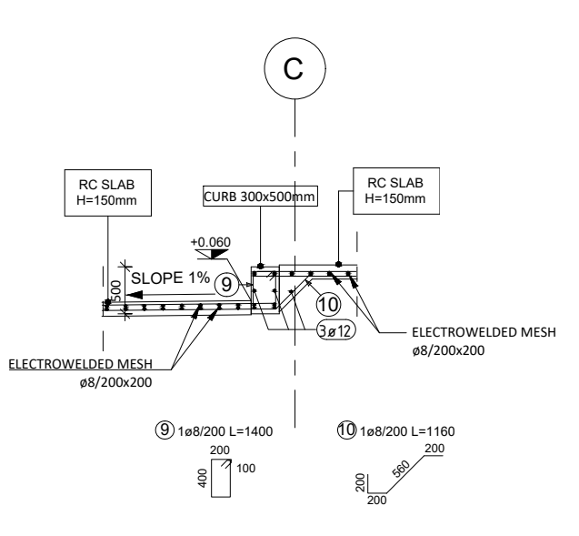
SECTION E-E 1:50
