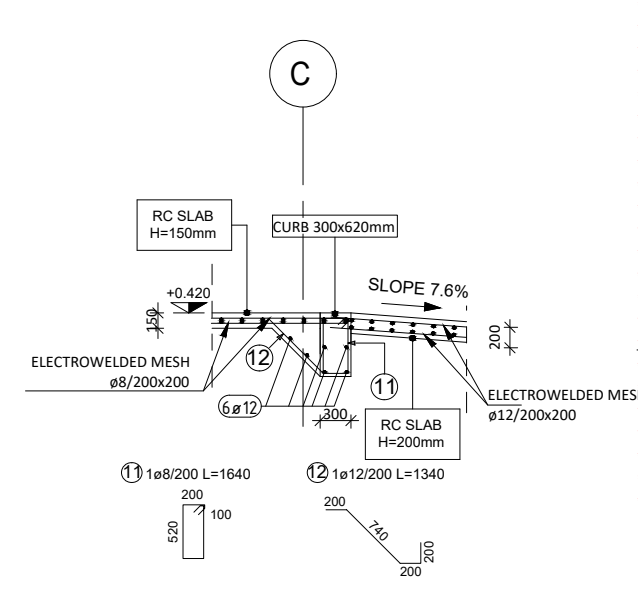
SECTION F-F 1:50
