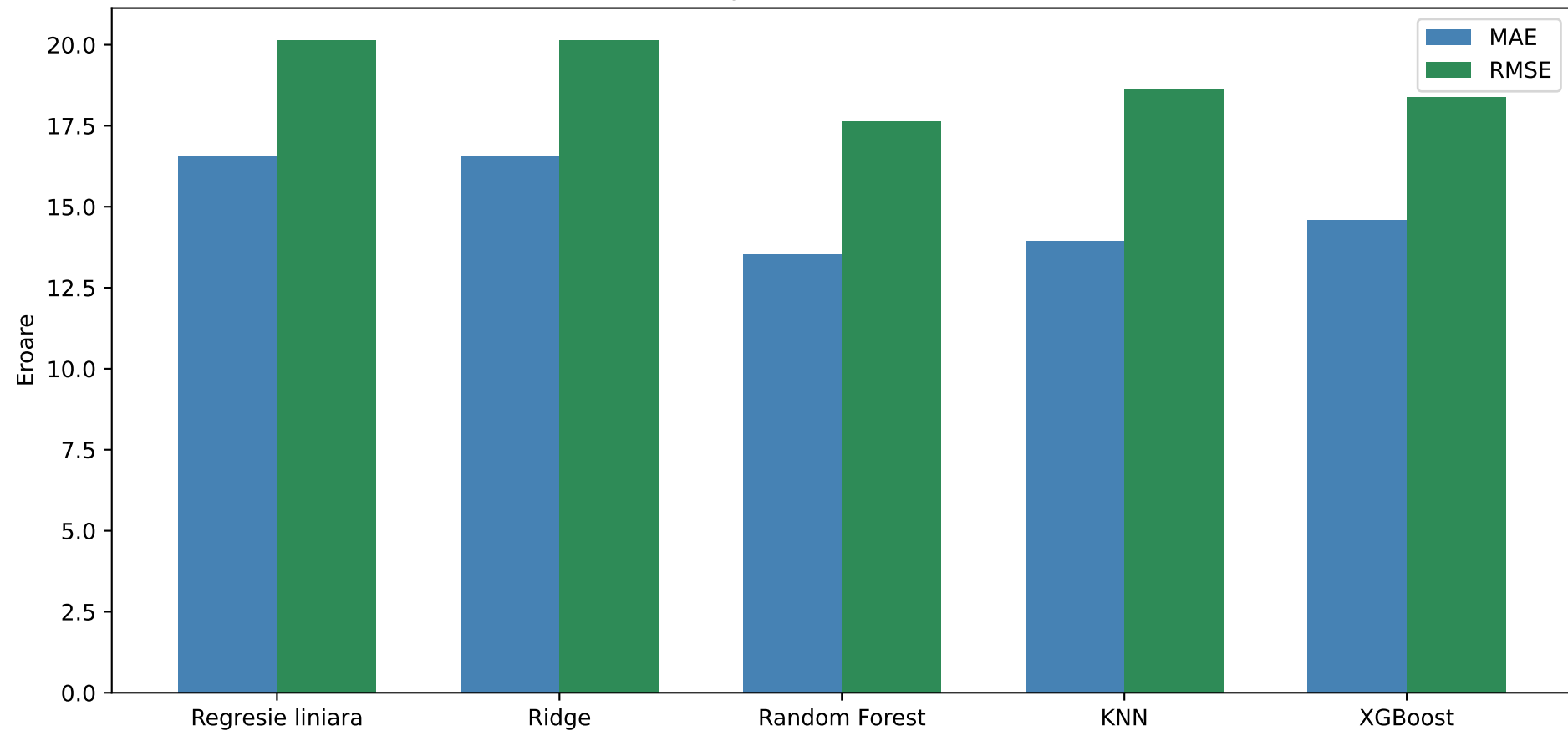
Comparatie MAE vs RMSE
