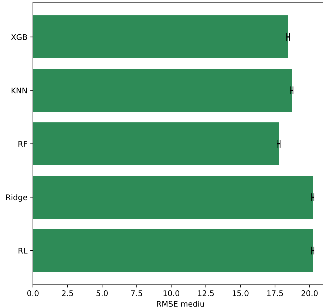
RMSE mediu +/- deviatie(10 rulari)
