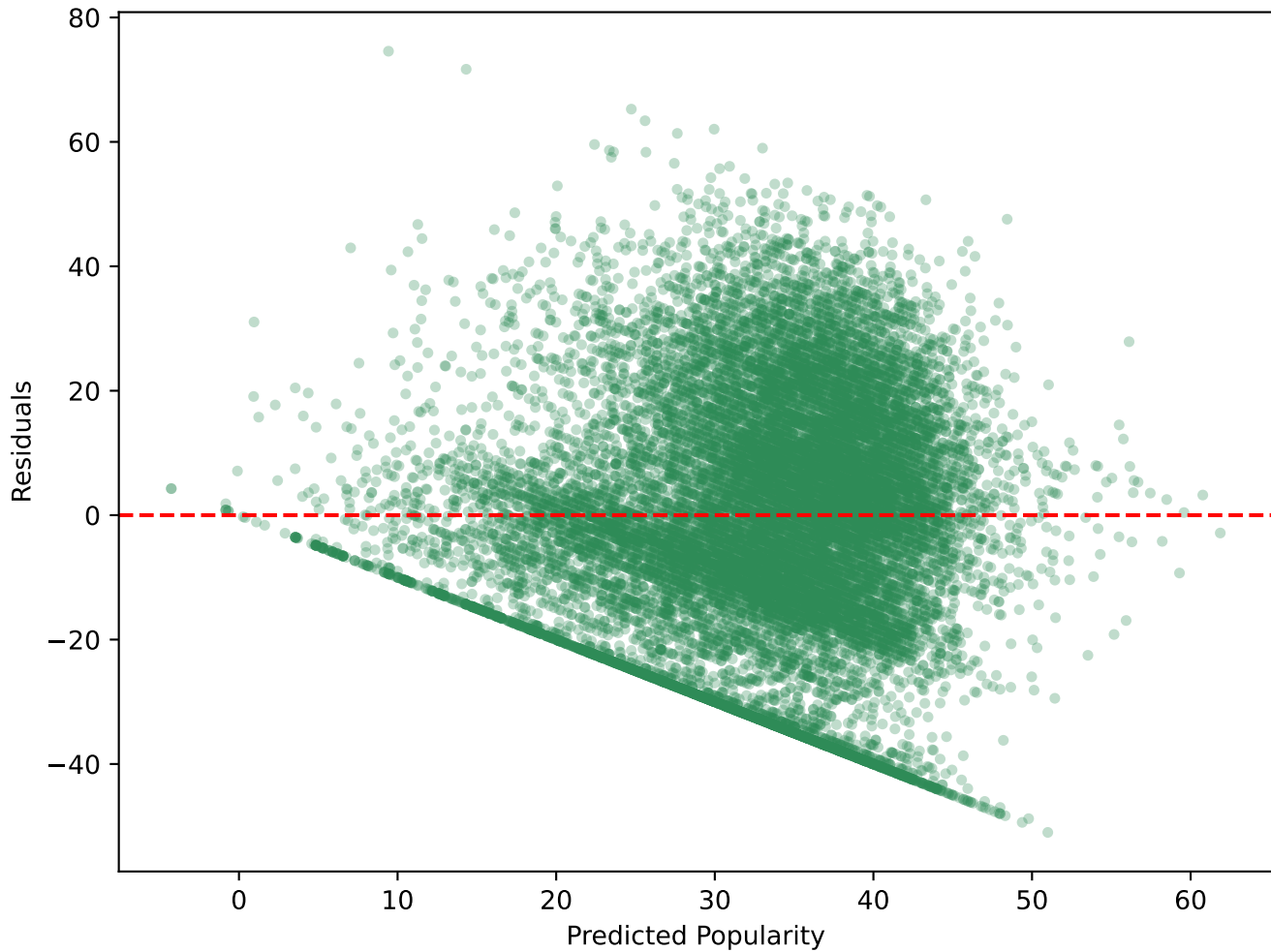
Residual Plot-XGBoost
