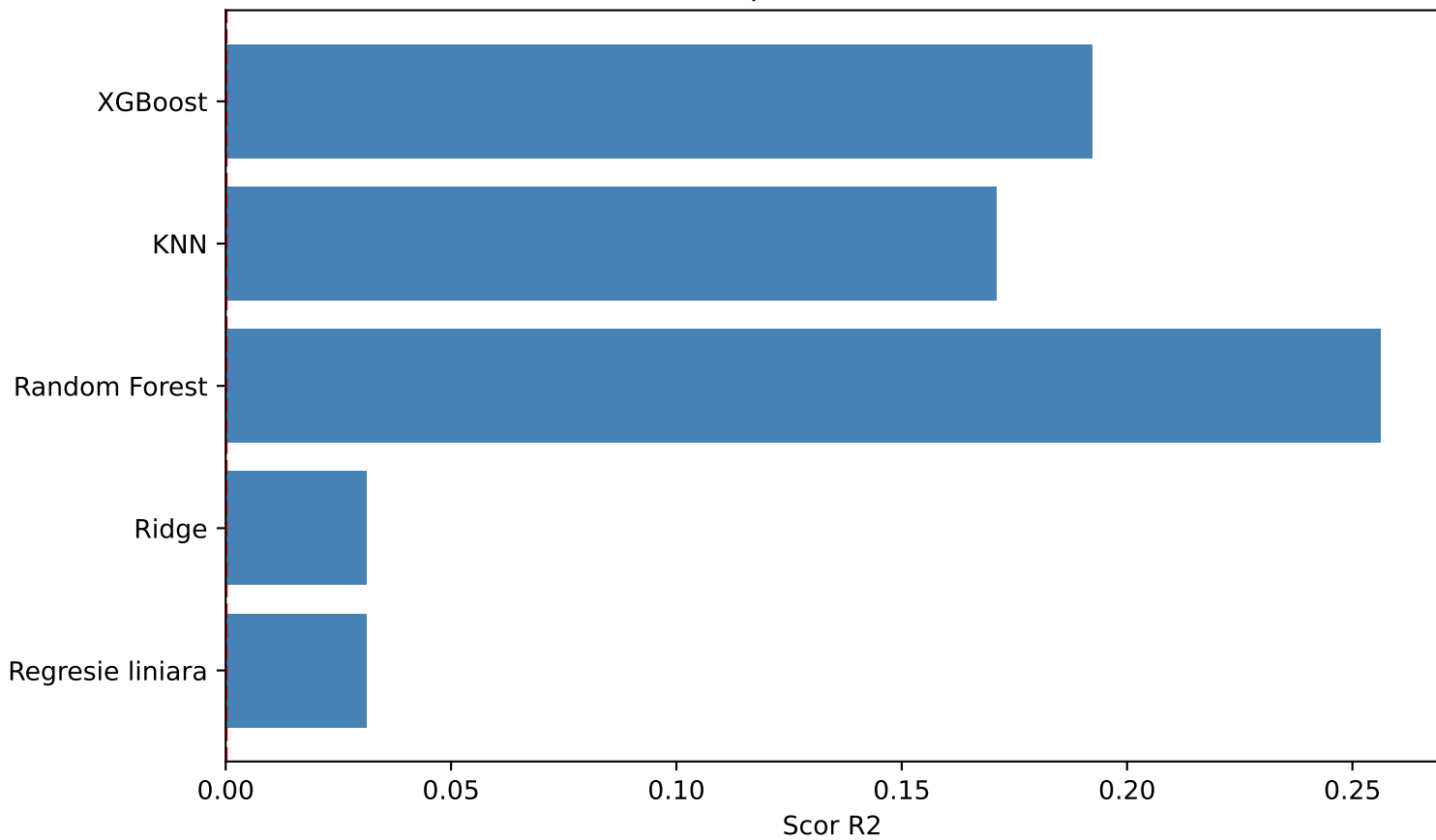
Comparatie scor R2
