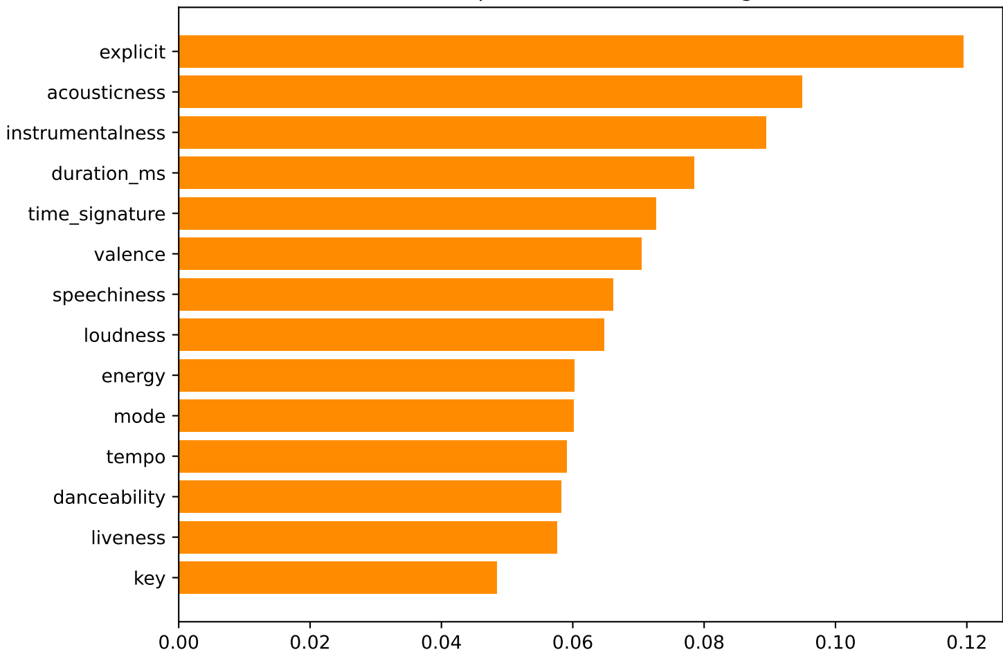
Feature importances - XGBoost Regressor
