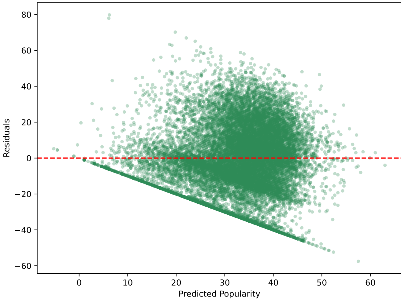
Residual Plot-XGBoost
