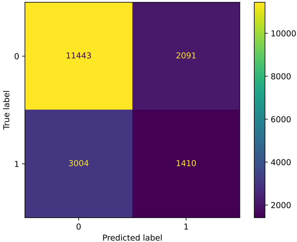
Confusion Matrix KNN
