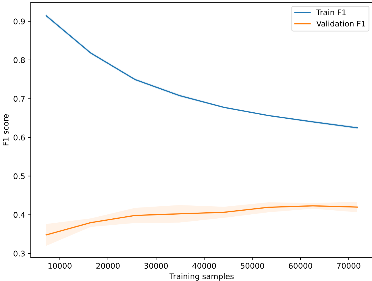
Learning curve - XGBoost
