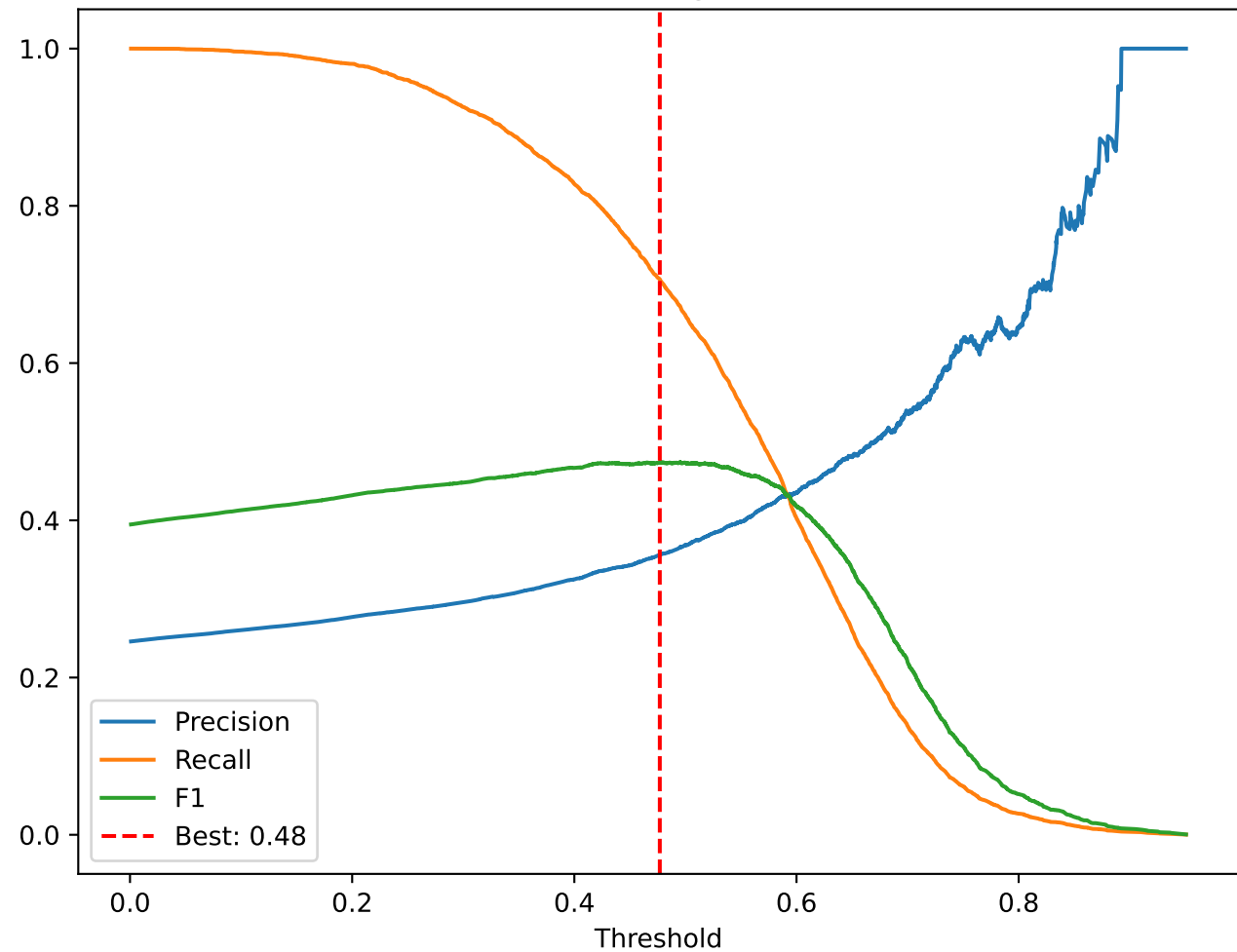
Threshold Tuning - XGBoost
