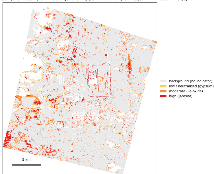
Figure 4. Scene-relative acid-generating-potential screening at Bingham.
