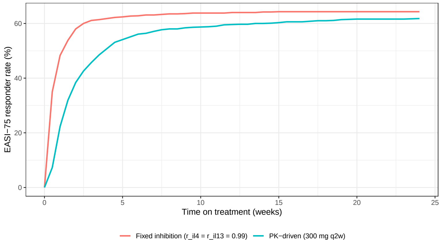
Fixed inhibition vs. PK-driven inhibition, same virtual patients, matched 300 mg dose
