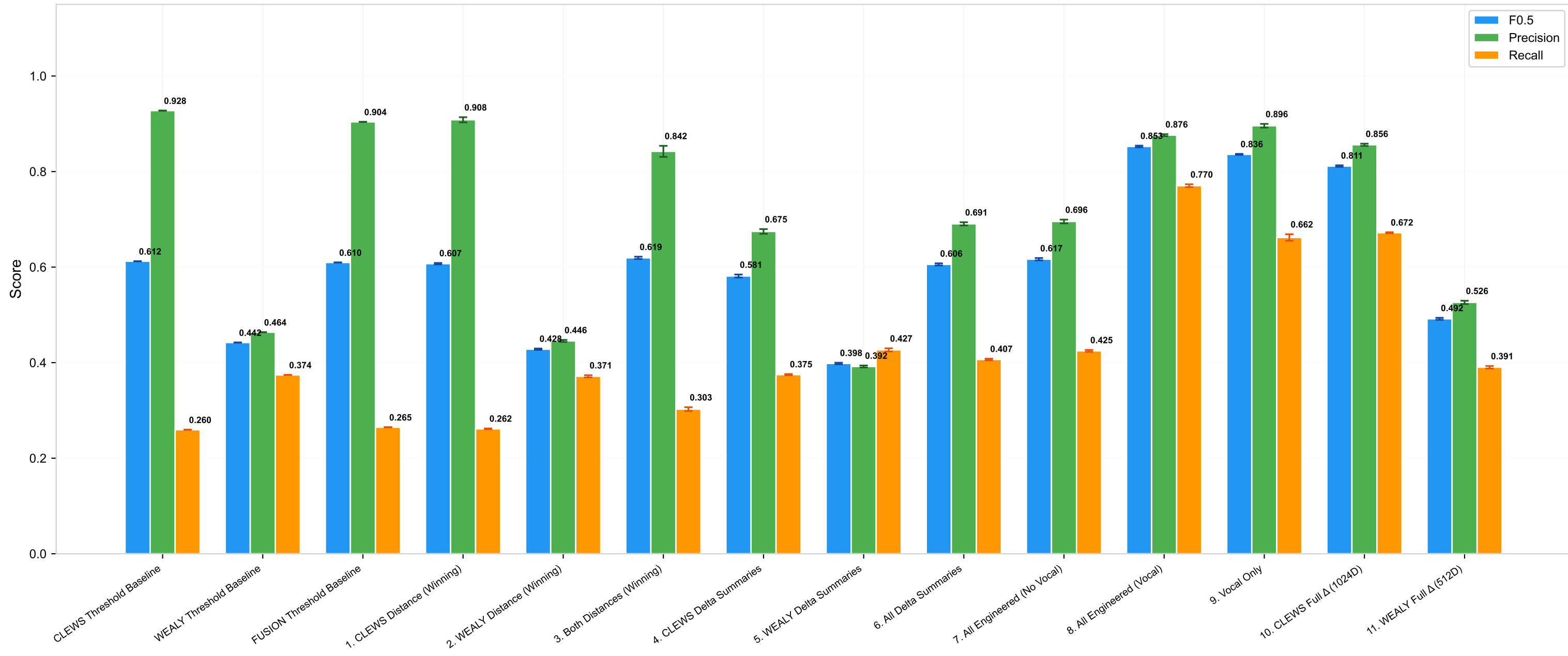
Feature Ablation: Classification Performance (XGBoost, 10 seeds)
