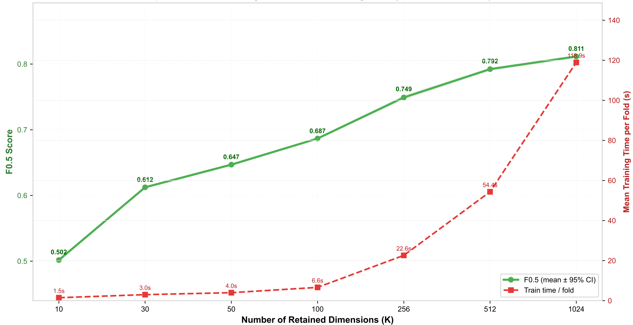
Top-K CLEWS Convergence: F0.5 & Training Cost (10 seeds, \pm 95\% CI)
