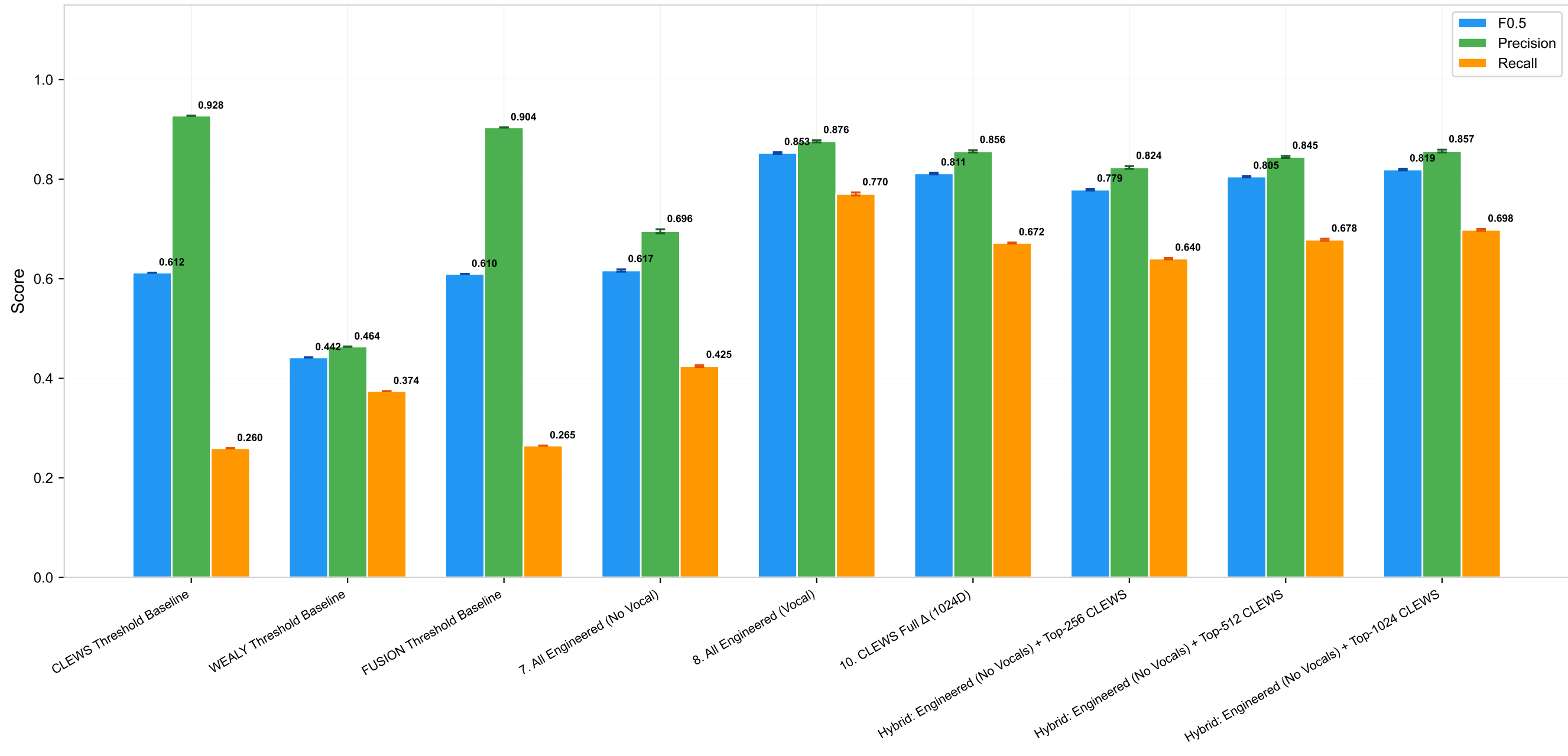
Hybrid Experiments: Engineered + Top-K CLEWS Dimensions (10 seeds, \pm 95\% CI)
